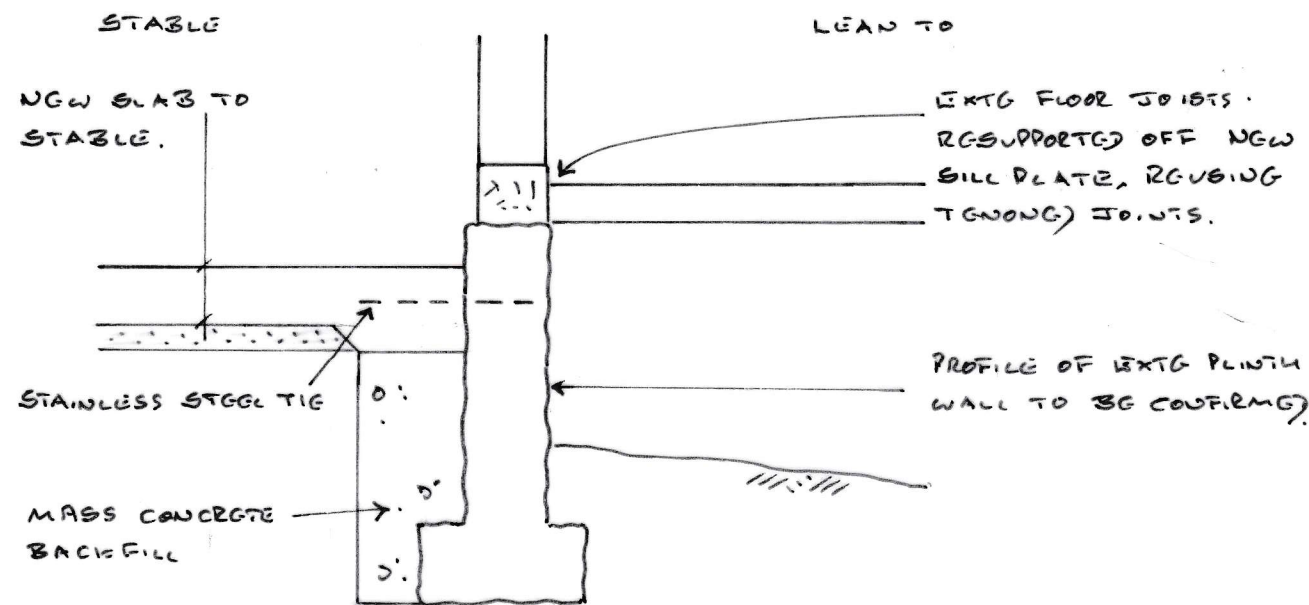
DETAIL 6-6
