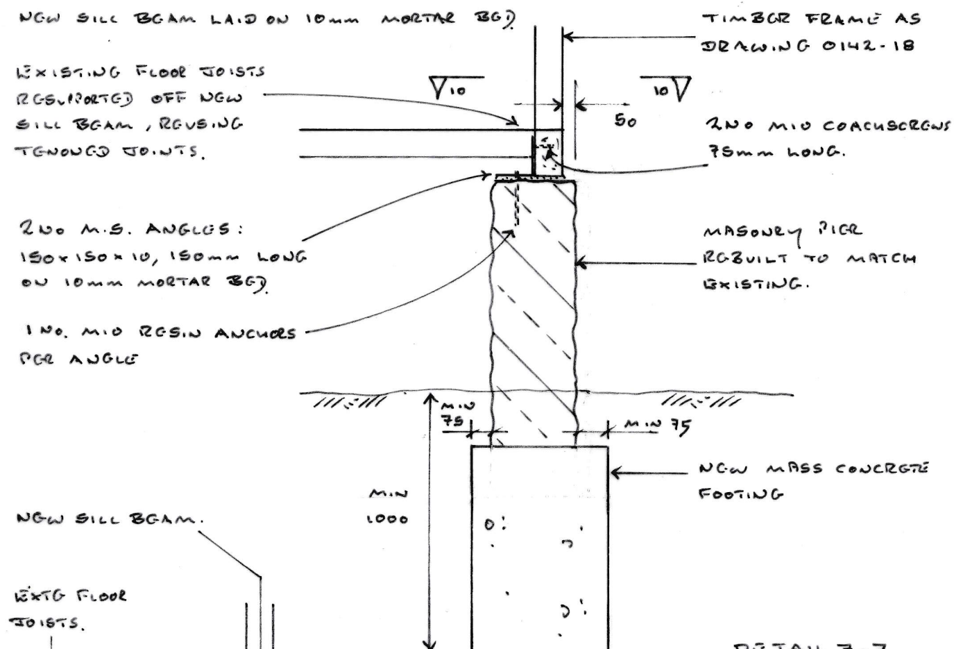
DETAIL 7-7
