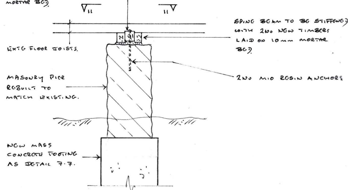
DETAIL 8-8
