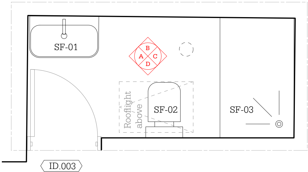
1 - Bathroom - Plan 1:25
