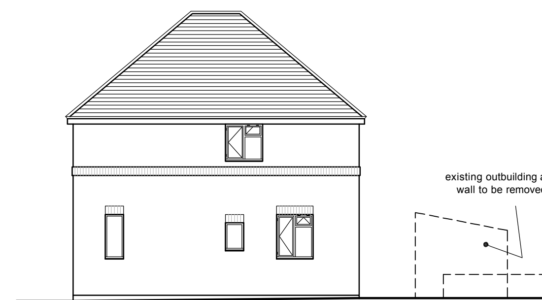
Existing South (side) Elevation
