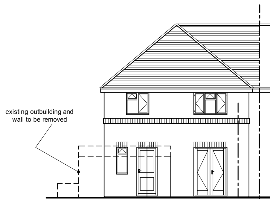
Existing East (rear) Elevation
