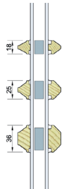
GLAZING BARS
