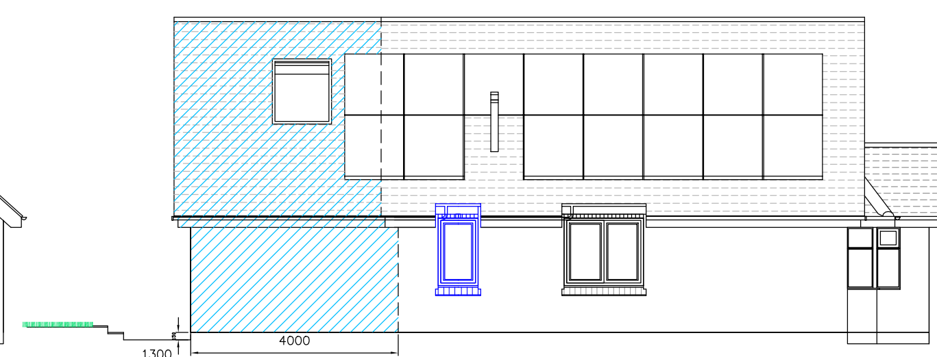
Proposed Side (South) Elevation
