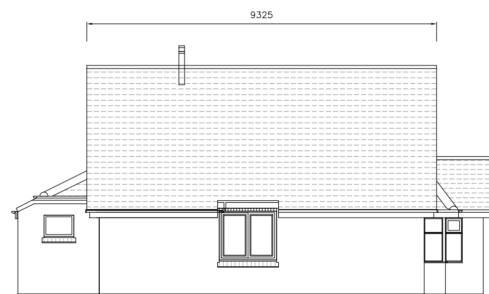
Existing Side (South) Elevation
