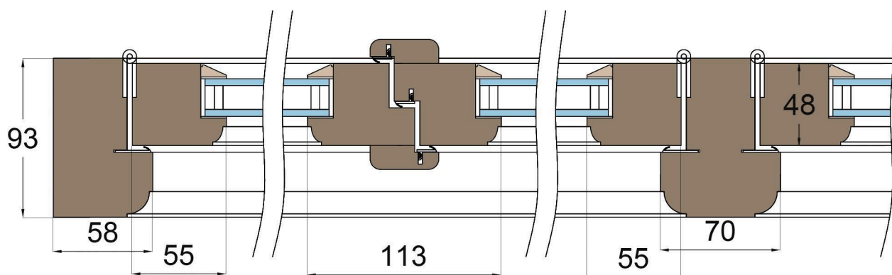
MULLION
