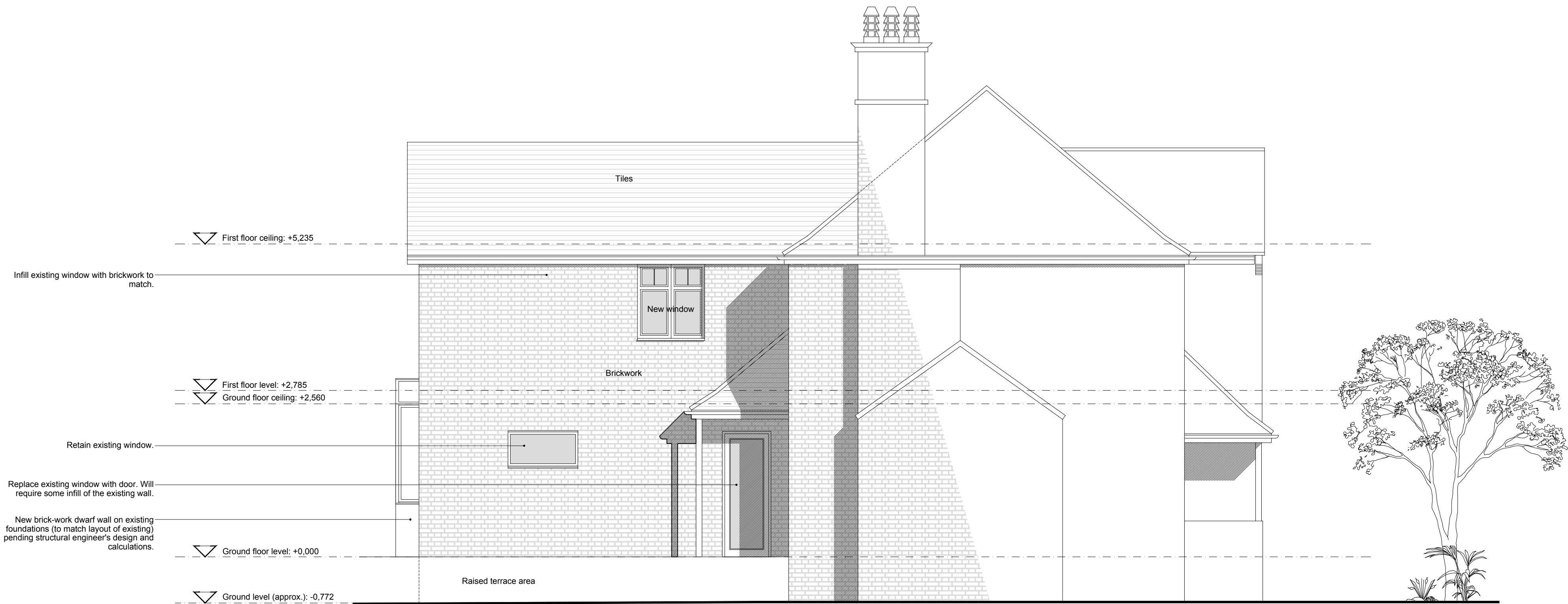
PROPOSED ELEVATION 2 Scale 1:50 at A1 0mm 1,000mm 2,000mm
