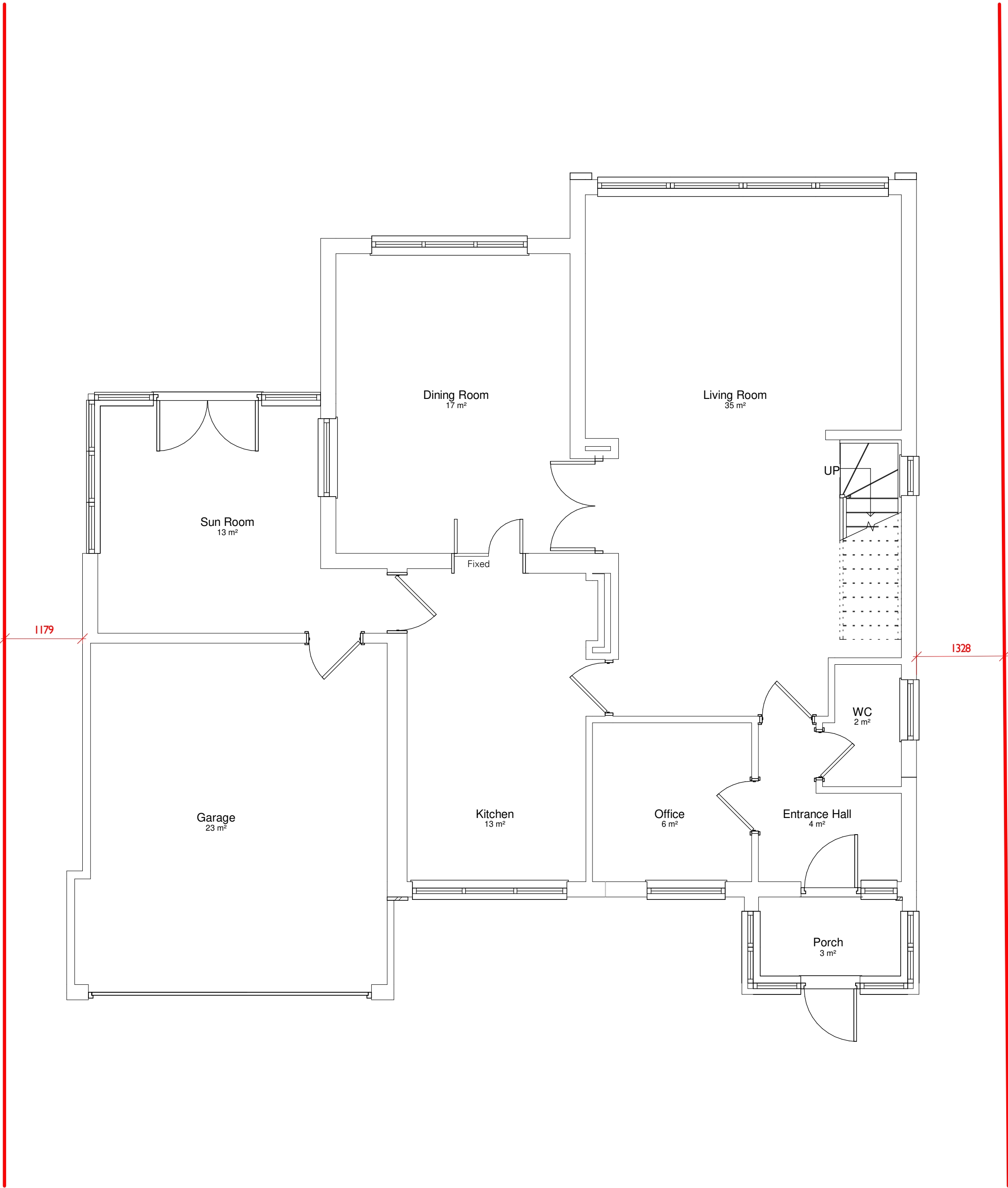
Existing_Level 00 1 : 50
