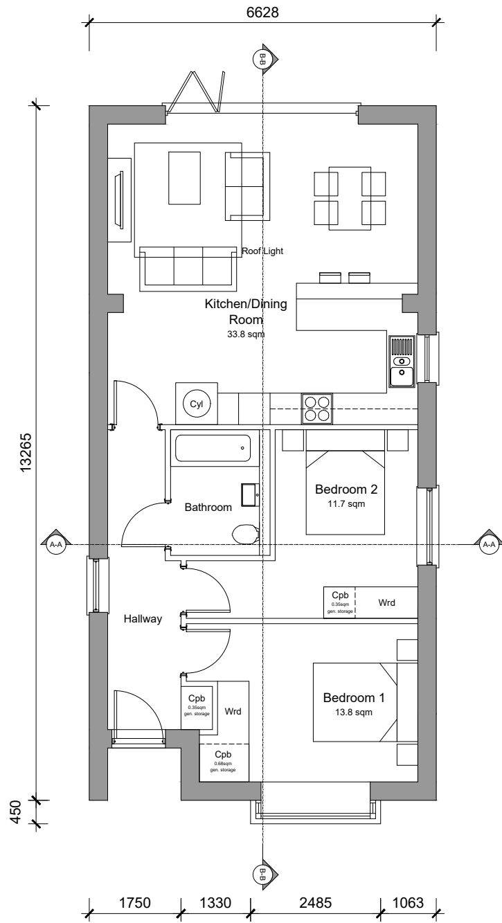
Ground Floor Plan 72.52sqm/781sqft
