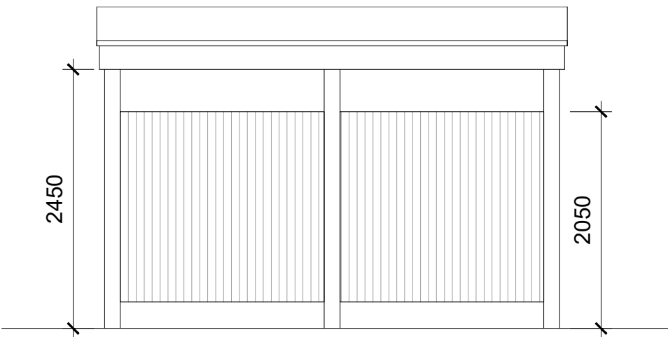
Rear Elevation
