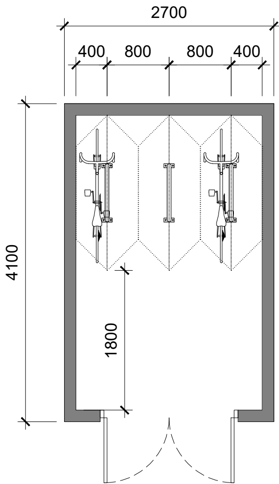
Cycle Store Plan
