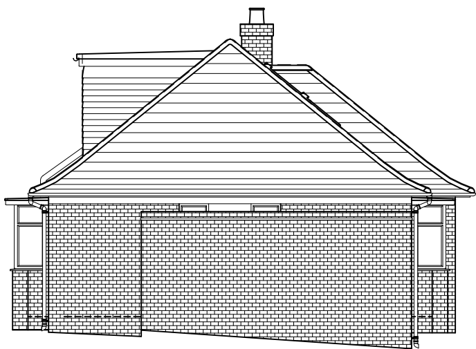
EXISTING LEFT SIDE ELEVATION
