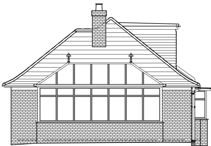
EXISTING RIGHT SIDE ELEVATION
