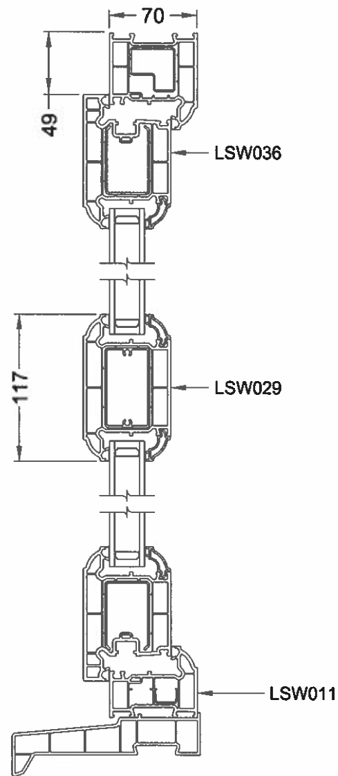
Section 'Y-Y'
