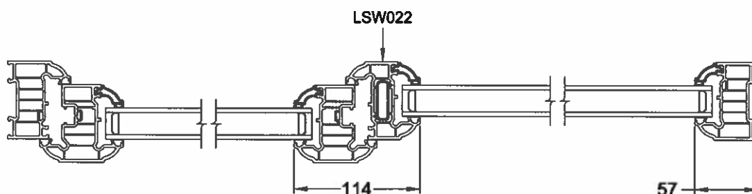
Section 'X-X'
