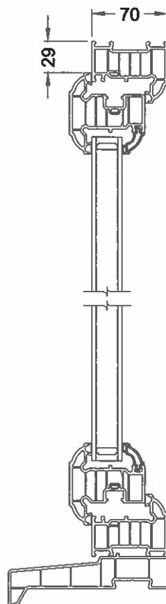
Section 'Y-Y'
