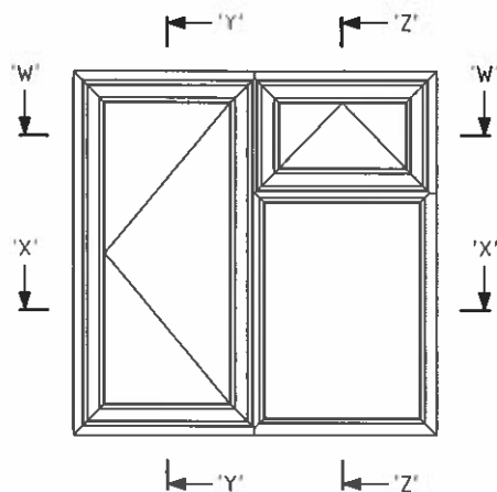
Typical Elevation (Viewed from outside)
