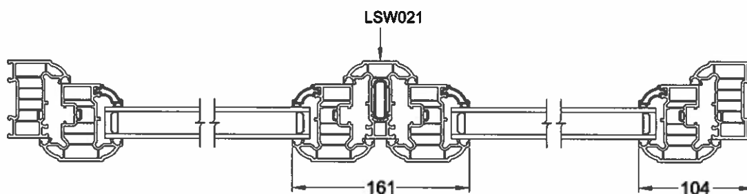
Section 'W-W'
