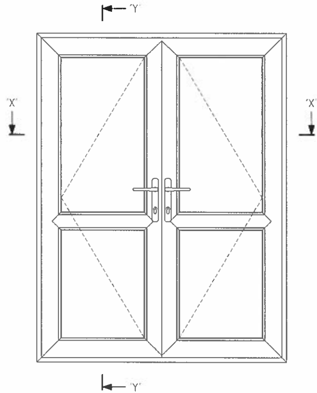
Typical Elevation (Viewed from outside)
