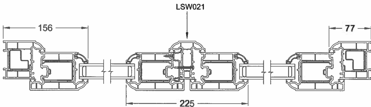
Section 'X-X'
