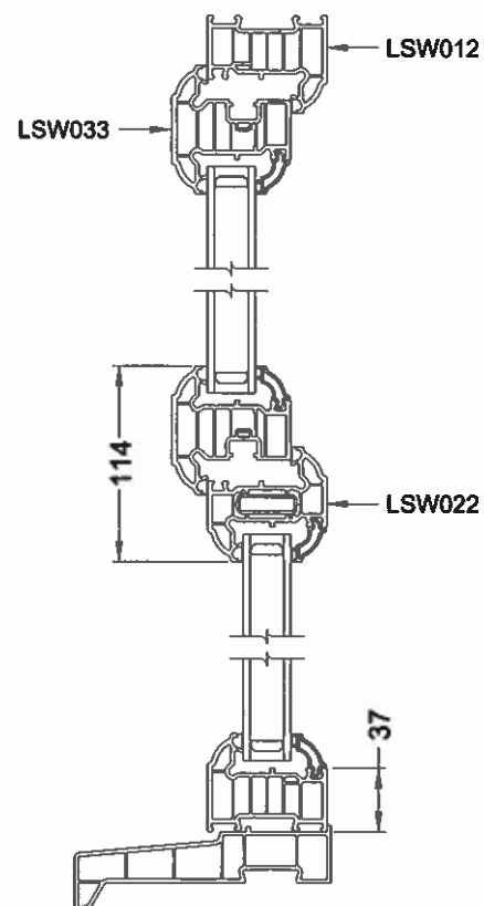
Section 'Z-Z'
