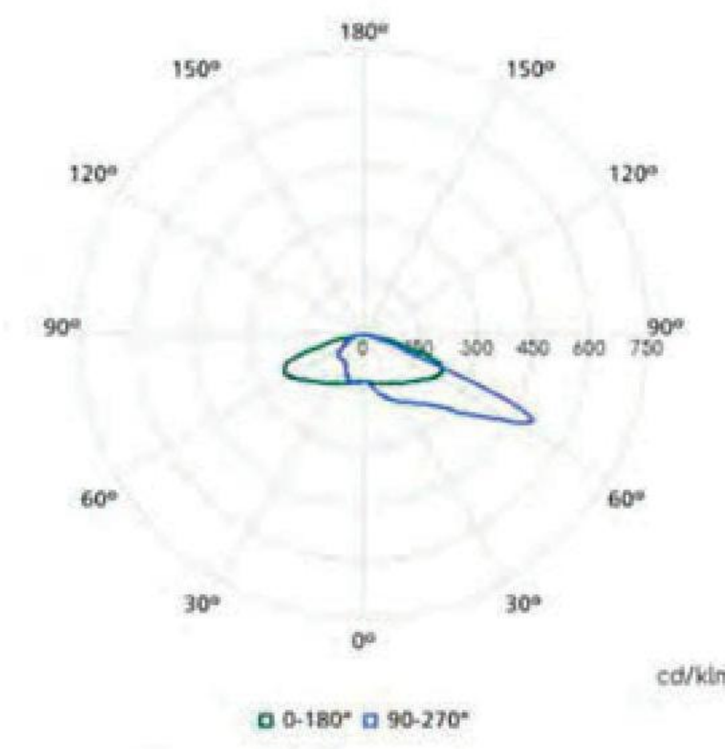
LumiStreet Gen2 Photometry
