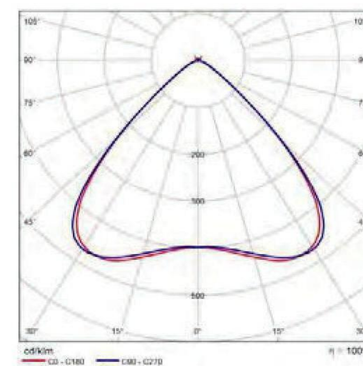
Pacific Gen 5 Photometry
