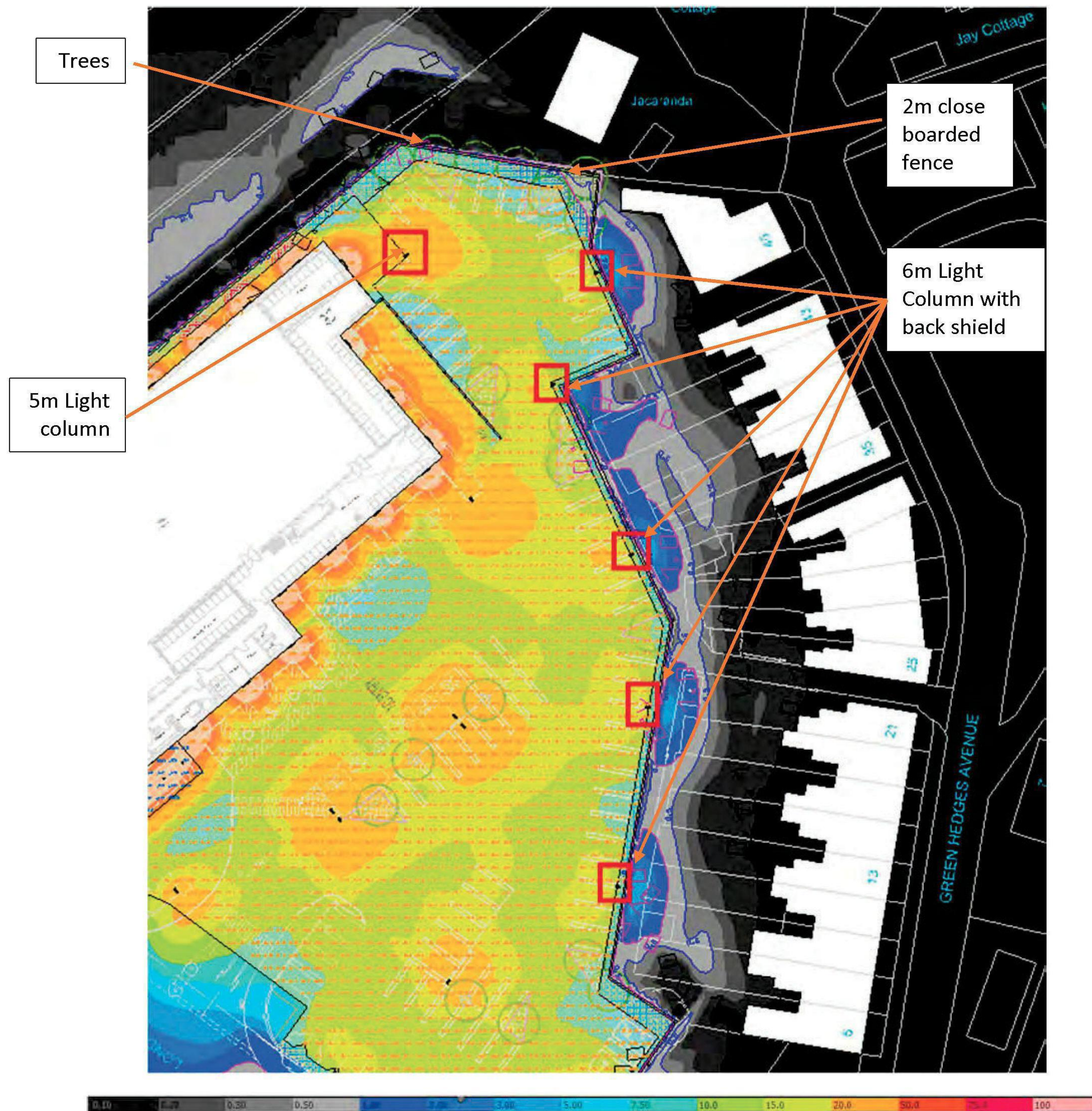
Figure 2 - Residential properties on Green Hedges Avenue in the lighting model. The light spill from the car park across the eastern site boundary is between 0.20 to 1 lux
