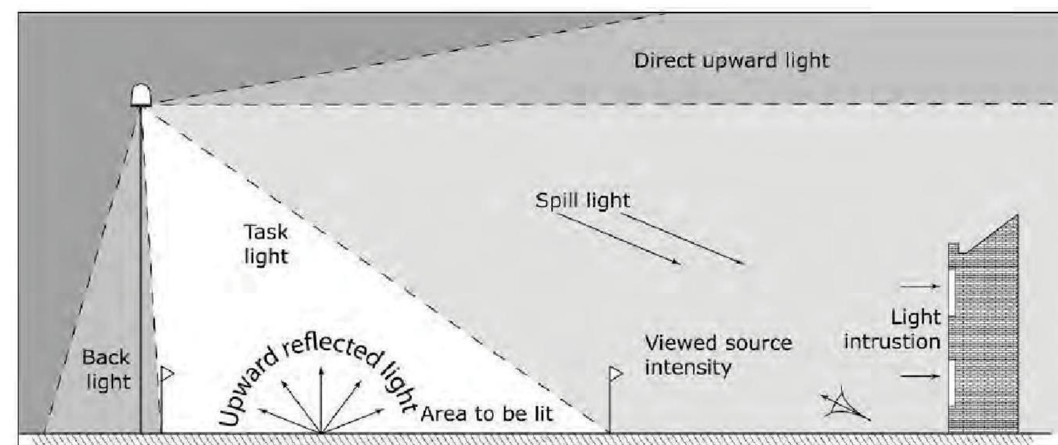
Types of obtrusive light
