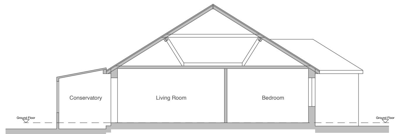
SOUTH SECTION/ELEVATION 1:100
