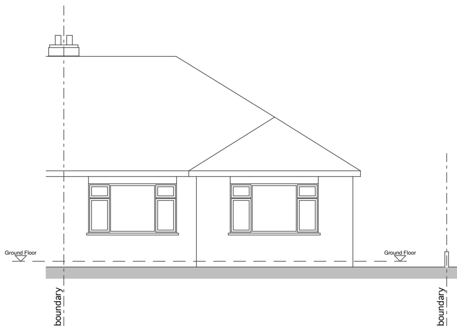
EAST ELEVATION 1:100
