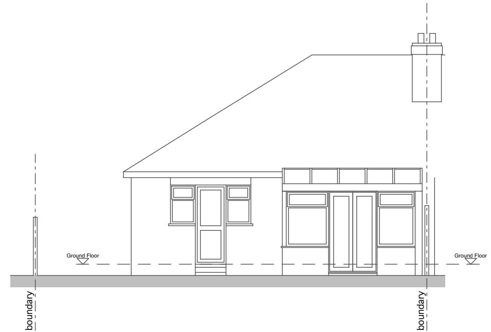
WEST ELEVATION 1:100
