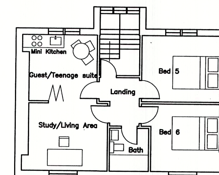
Second Floor Plan - Proposed
