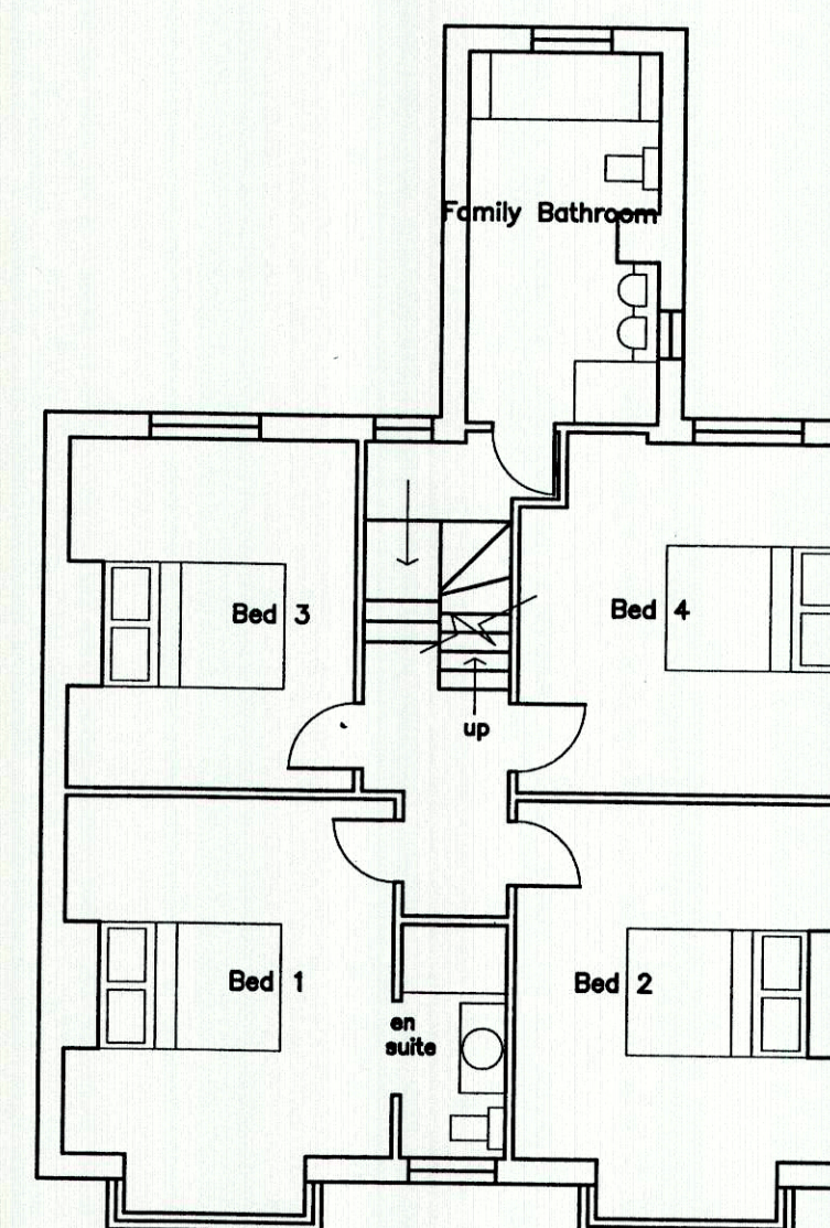
First Floor Plan - Proposed
