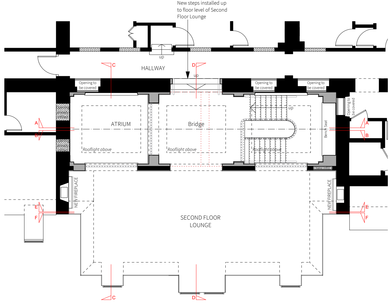
Proposed Second Floor Plan Part plan showing atrium space and second floor lounge. 1:100 @A3 / 1:50 @A1
