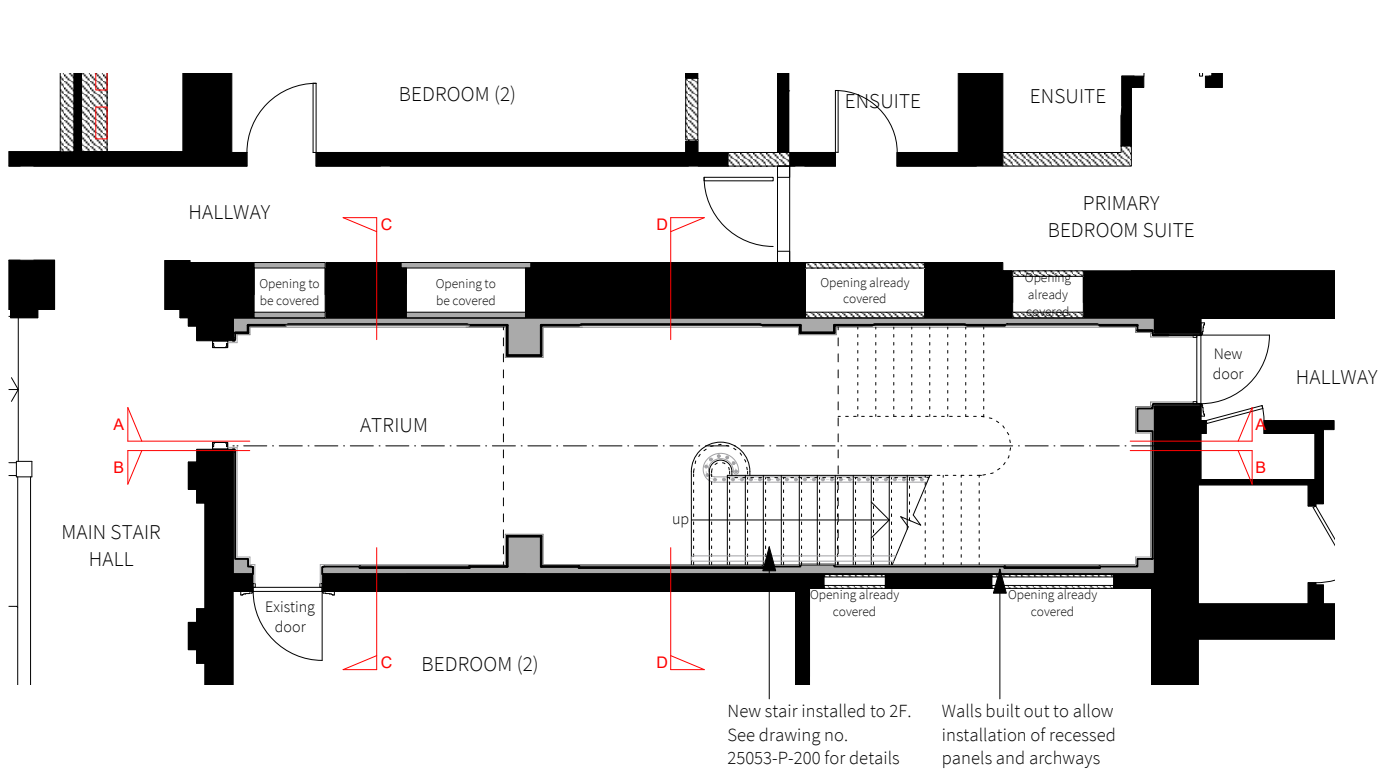
Proposed First Floor Plan Part plan showing atrium space. 1:100 @A3 / 1:50 @A1
