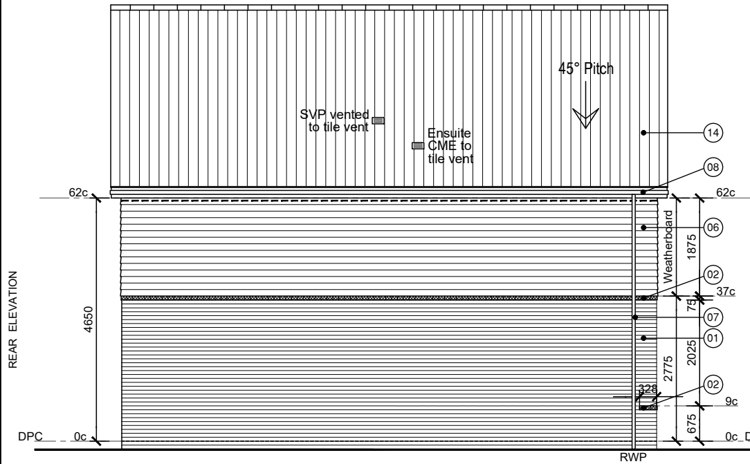
SIDE ELEVATION
