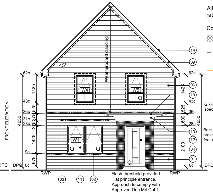
FRONT ELEVATION Plots : (AS) - (OPP) 131, 132
