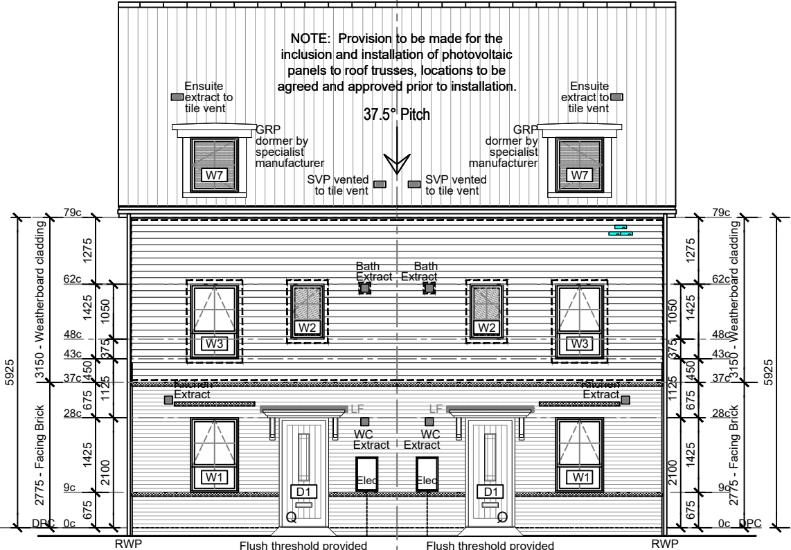
FRONT ELEVATION
