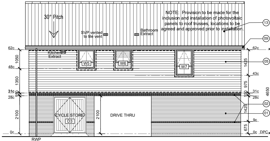
REAR ELEVATION
