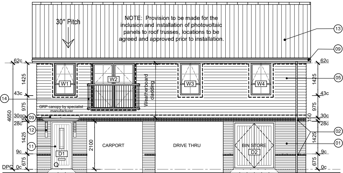
FRONT ELEVATION Plot 82
