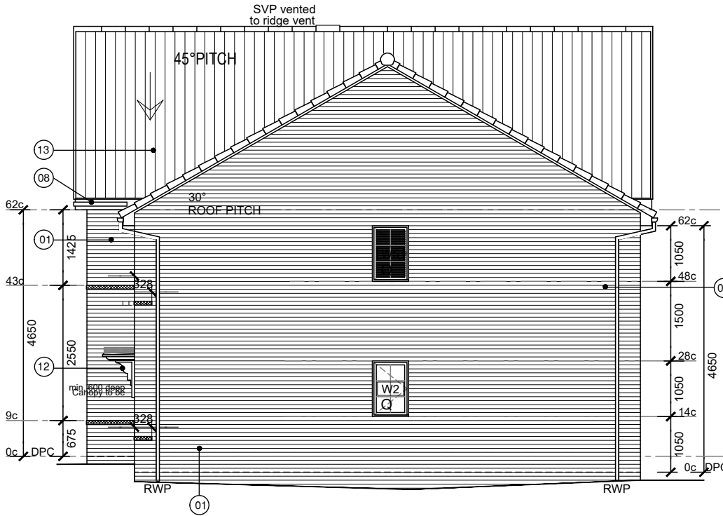
SIDE ELEVATION YB50 Plots 153
