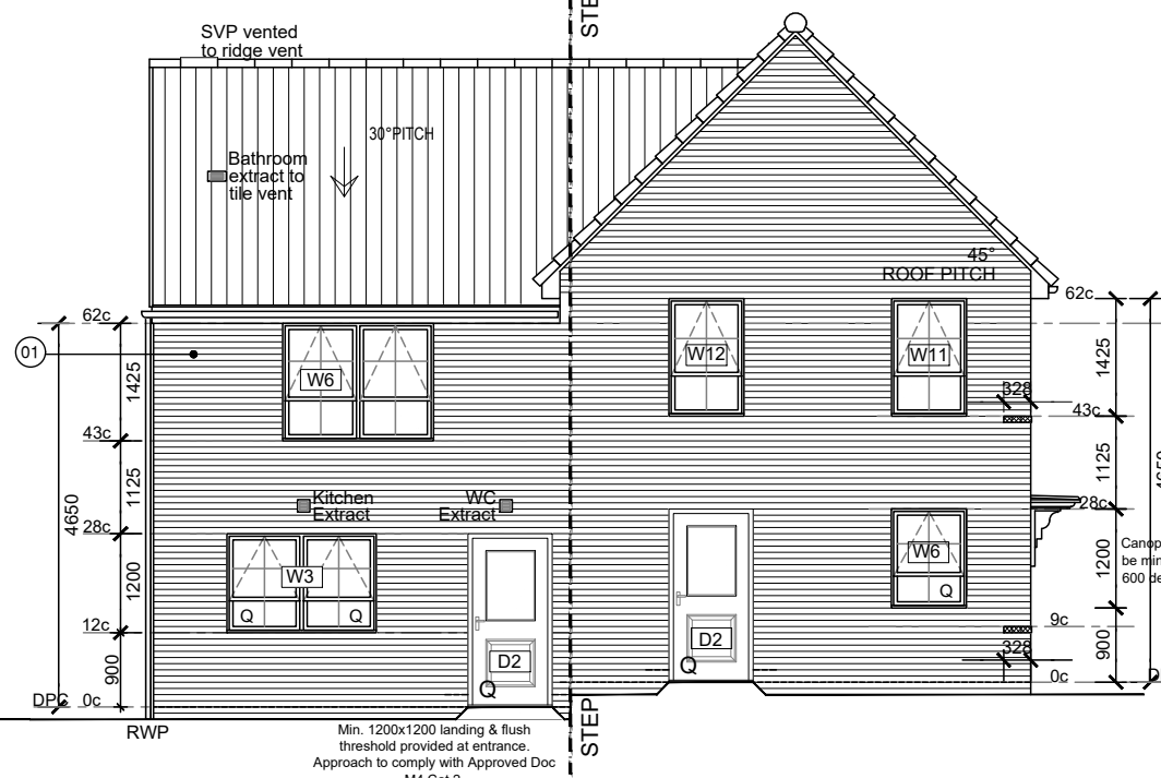
REAR ELEVATION YB55 Housetype Plots 153
