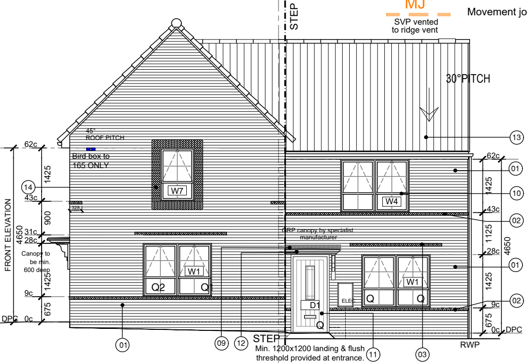
FRONT (YB50 ENTRANCE) ELEVATION YB55 Housetype Plots 154
