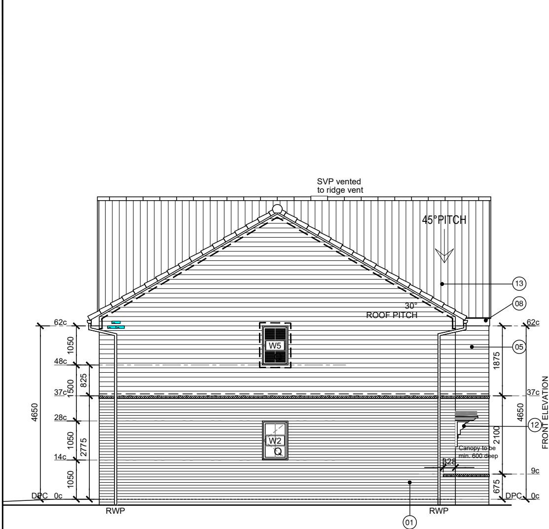
SIDE ELEVATION YB50 Plot 123
