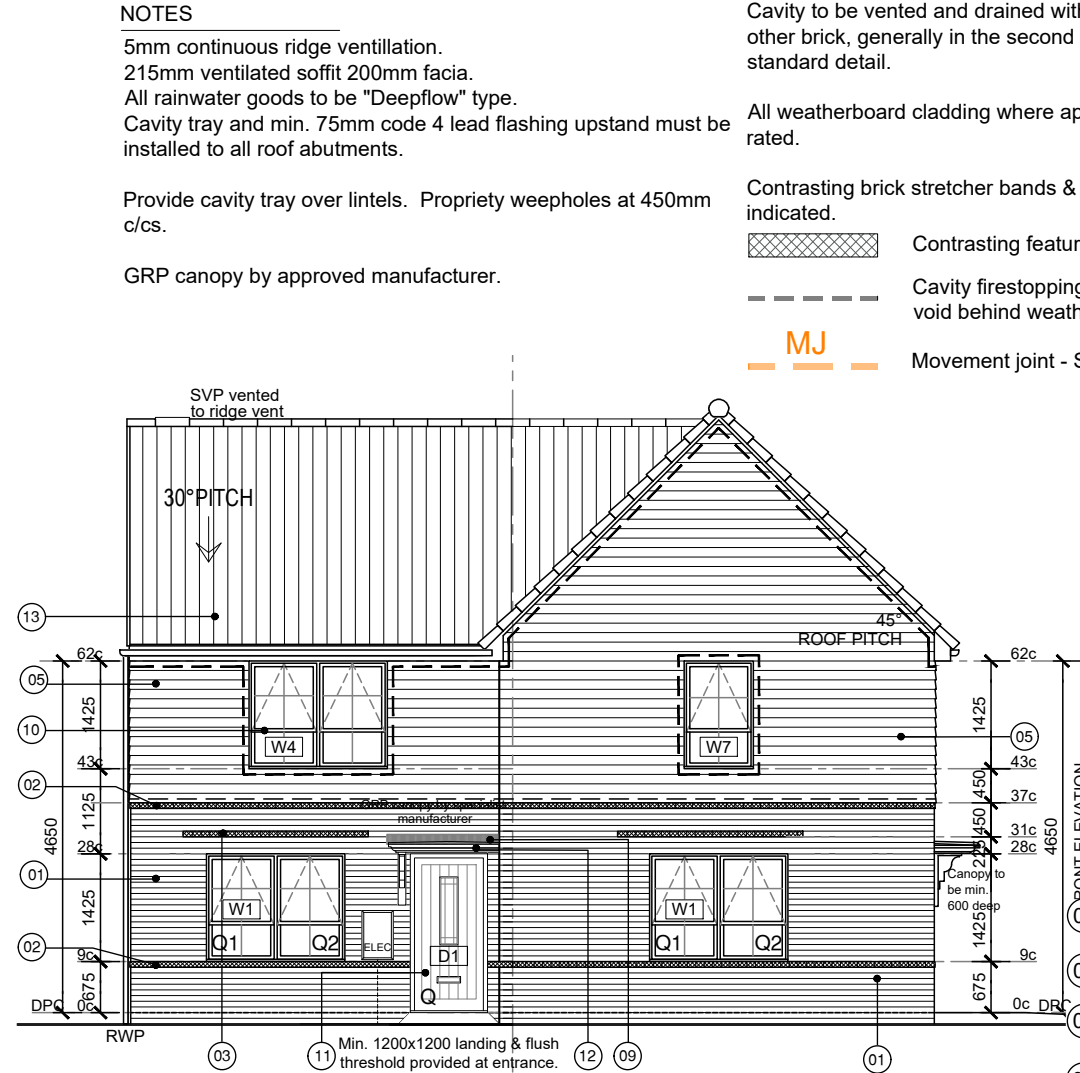
FRONT (YB50 ENTRANCE) ELEVATION YB50 Housetype Plot 123
