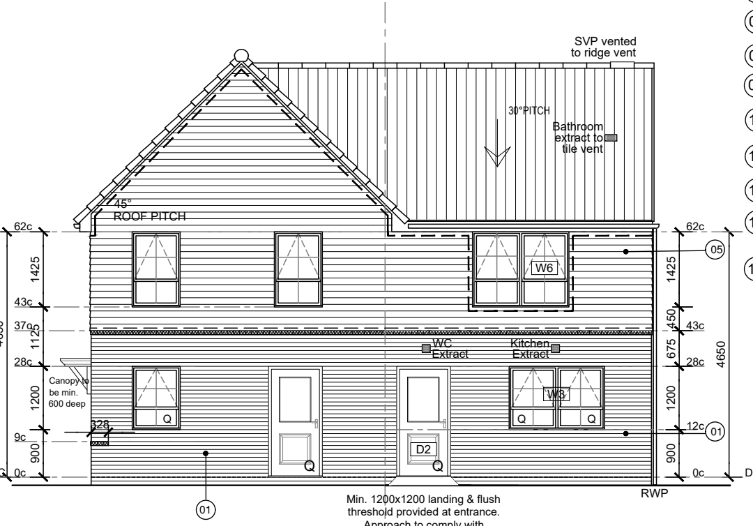
REAR ELEVATION YB55 Housetype Plot 122
