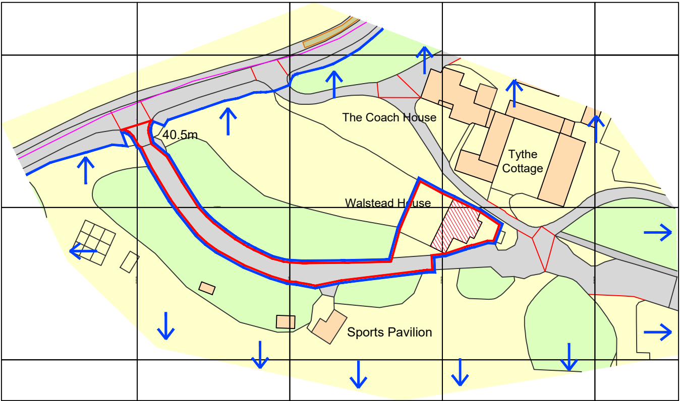
SITE LOCATION PLAN - AS PROPOSED SCALE @ 1:1250 ON AN A1 SHEET
