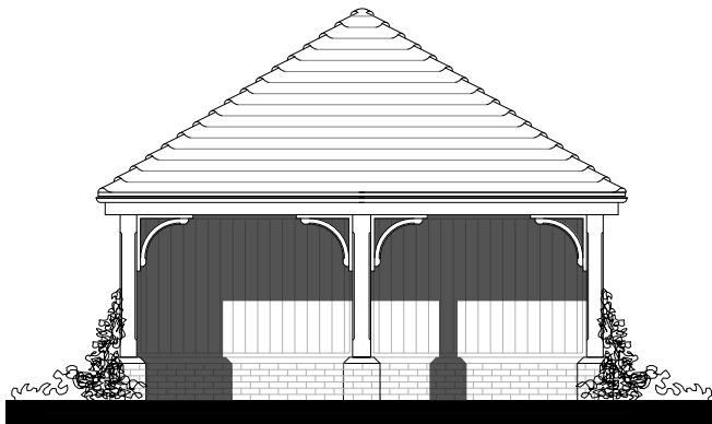
FRONT ELEVATION
