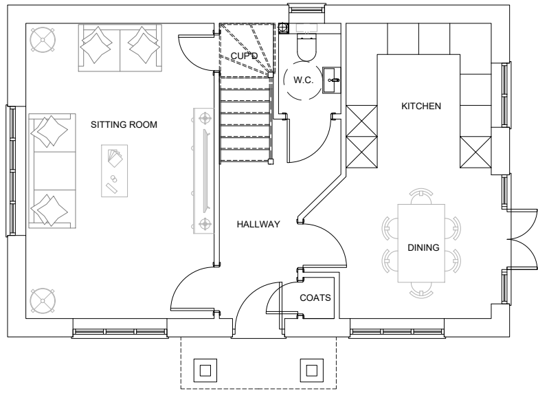
GROUND FLOOR PLAN 1096 SQFT
