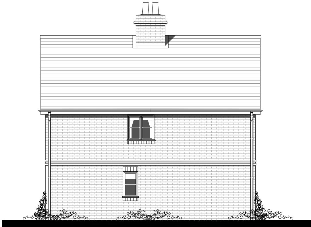
REAR ELEVATION
