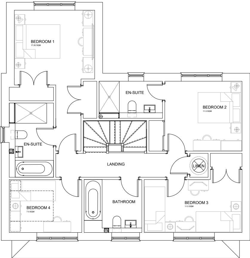
FIRST FLOOR PLAN PLOT 6
