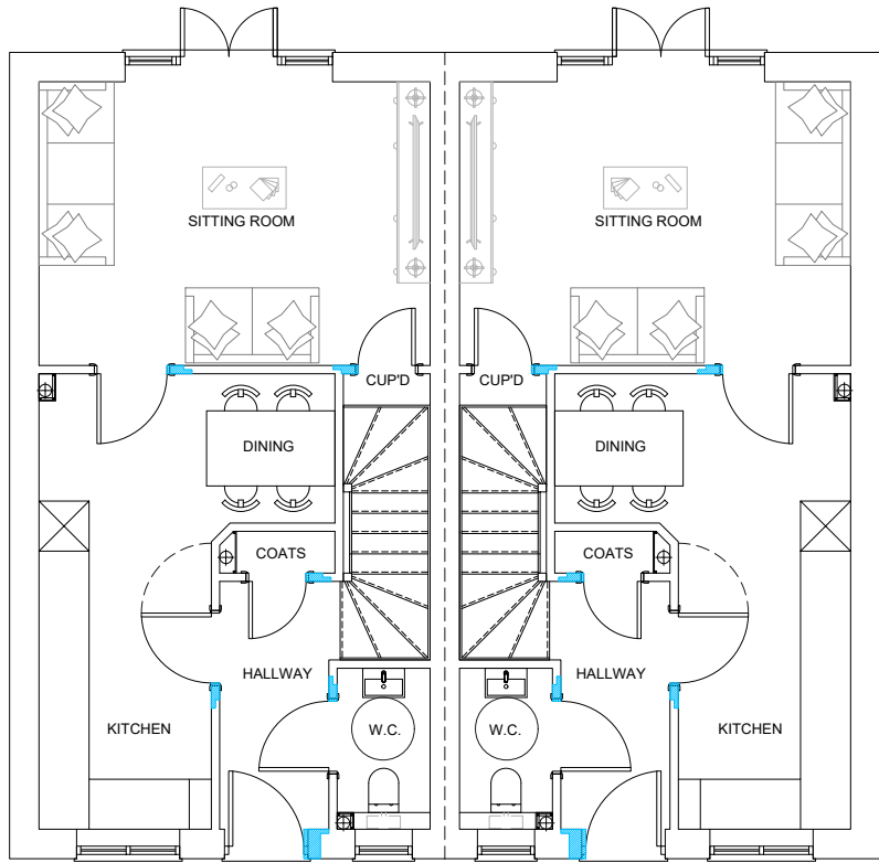
GROUND FLOOR PLAN 903 SQFT
