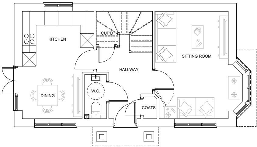
GROUND FLOOR PLAN PLOT 25 915 sqft
