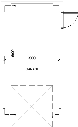
FLOOR PLAN
