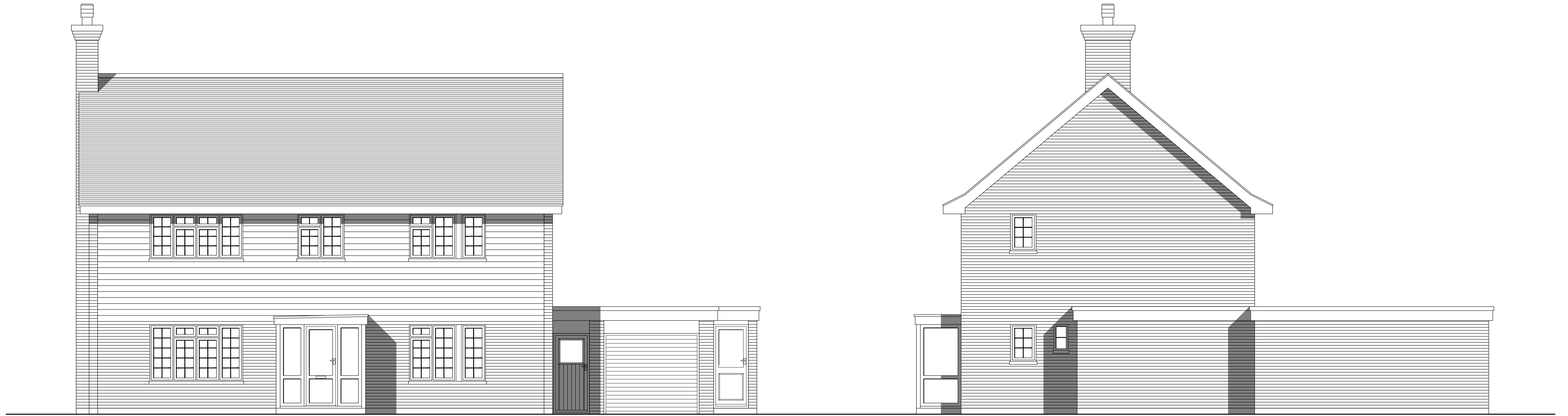
FRONT ELEVATION (EAST)
