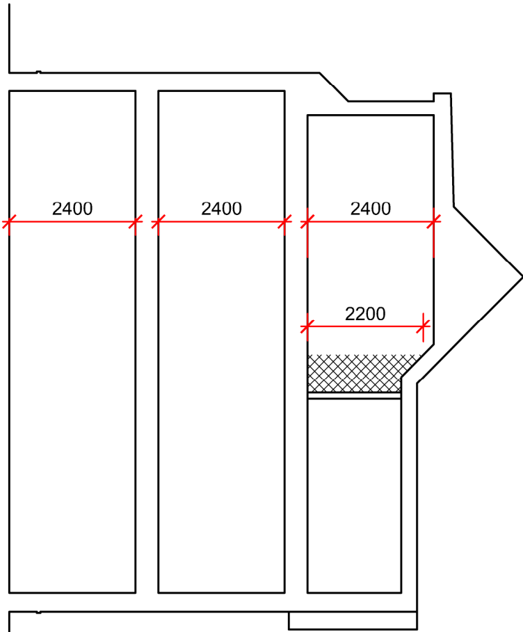
Typical Section A
