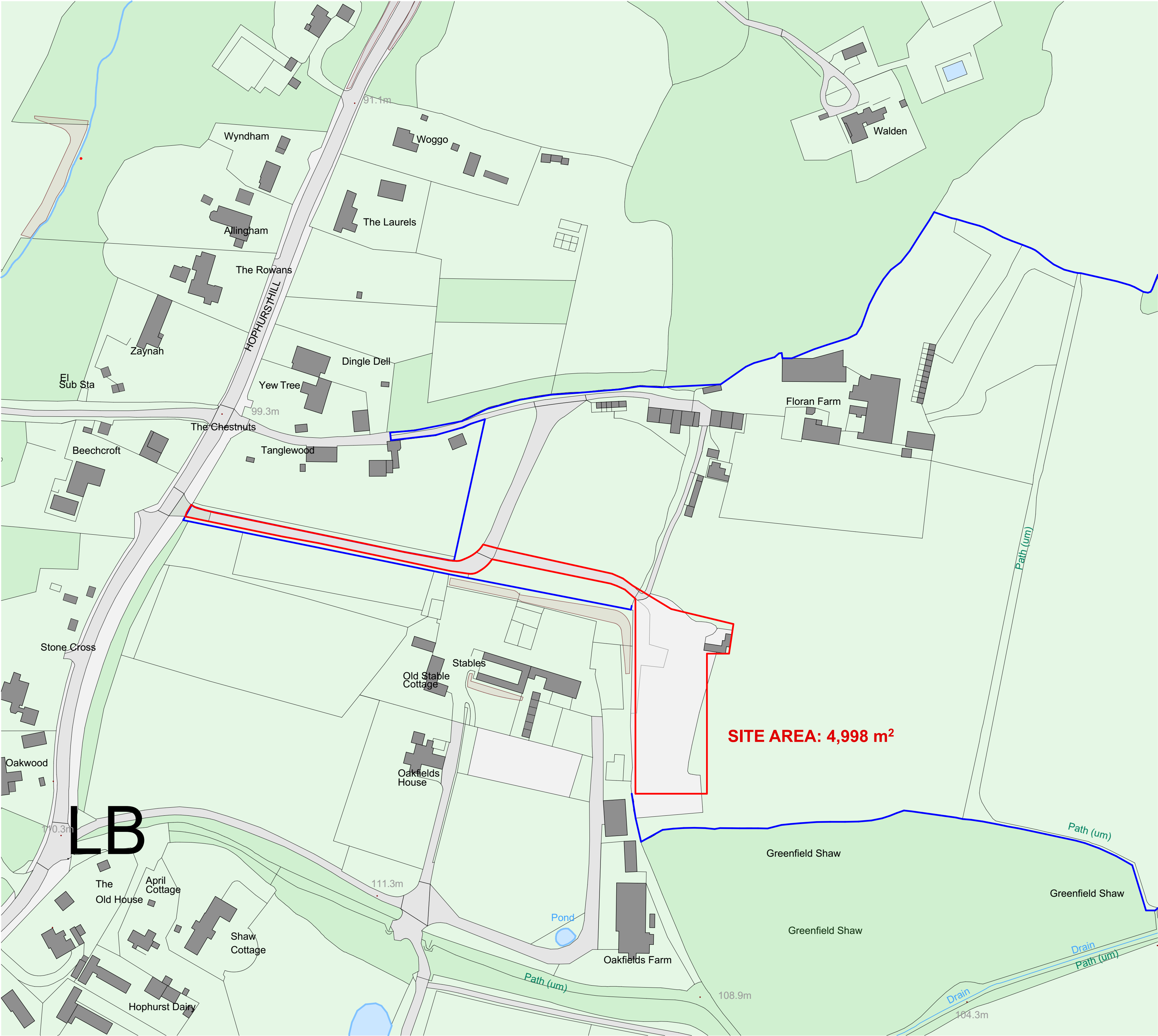
0. Location Plan 1:1250
