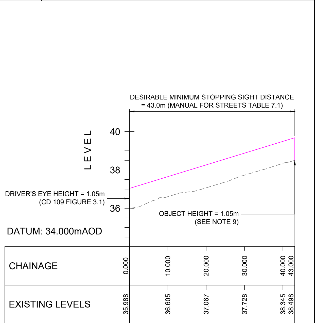
JUNCTION VISIBILITY SOUTH 30MPH SCALE: H 1:500, V 1:100, 5x VERTICAL EXAGGERATION
