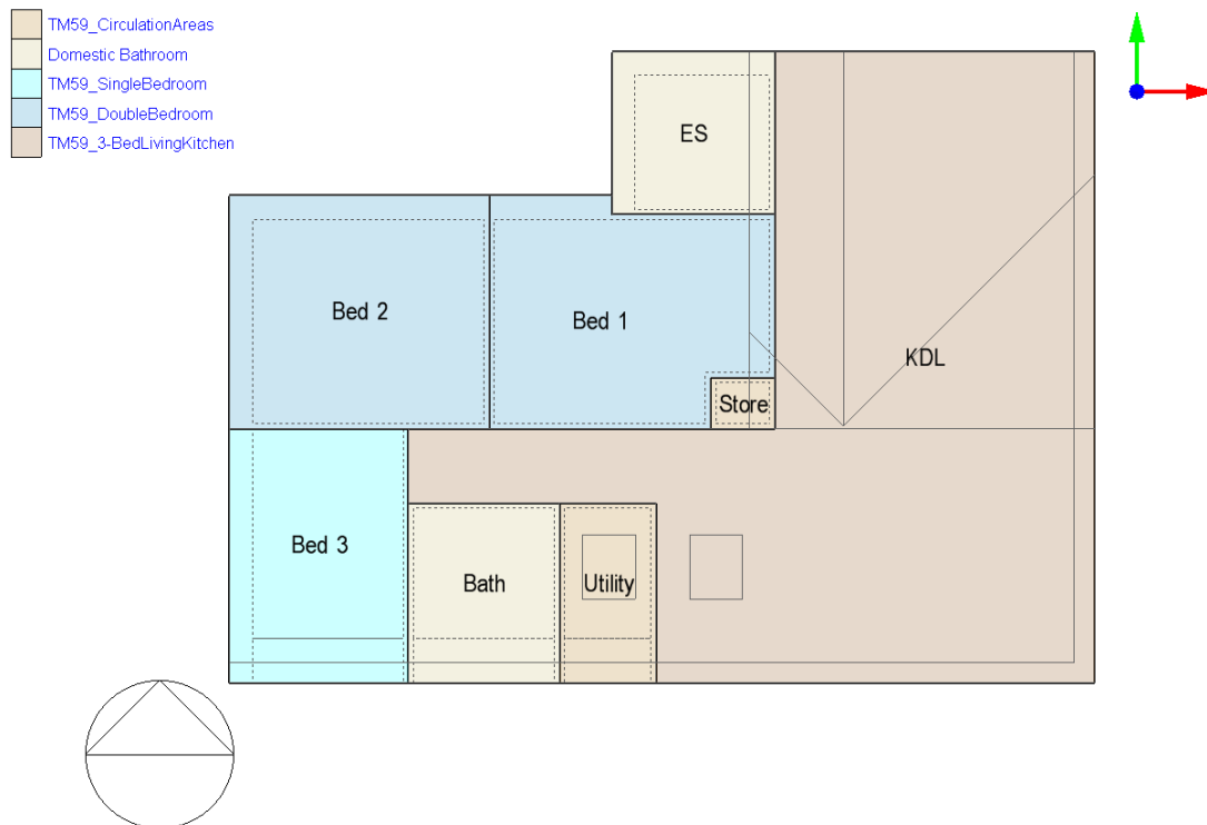
Figure 3 – internal zone layout:
