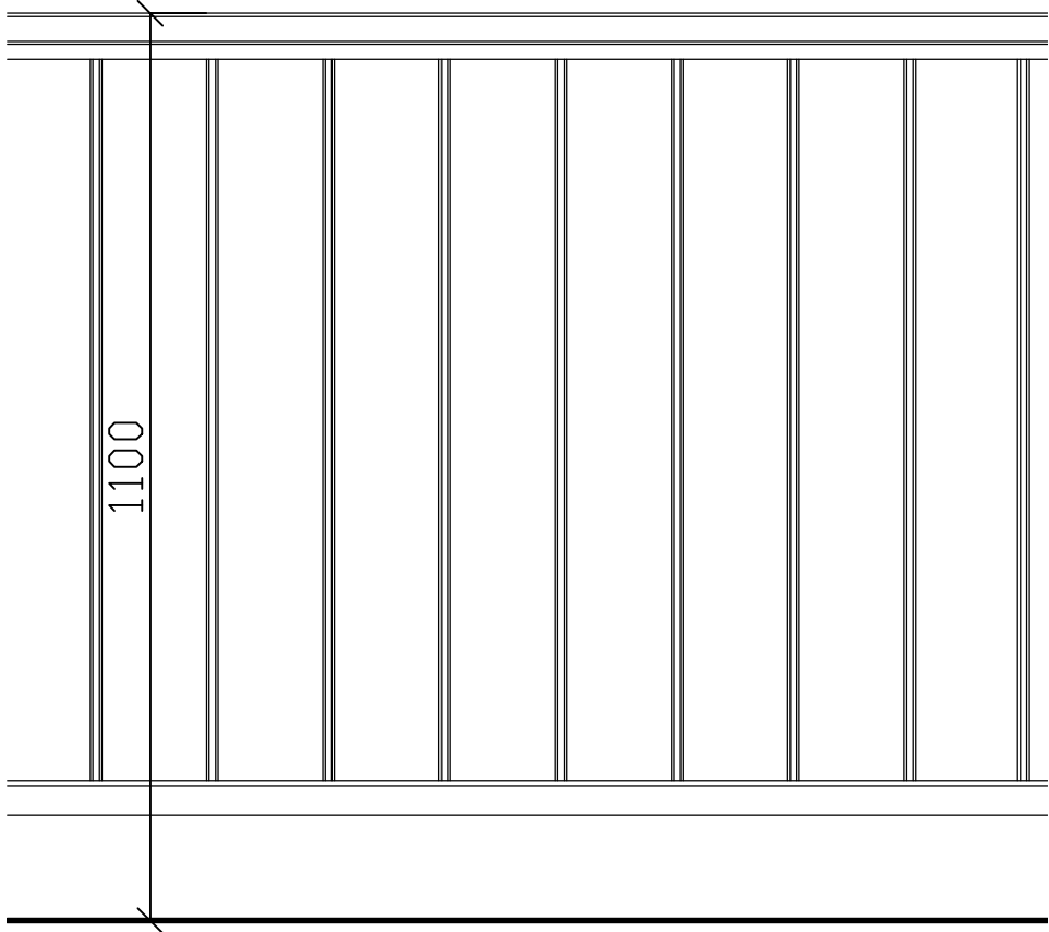
ELEVATION to BEAD and BUTT WALL BOARDING - Scale 1:10 @ A1
