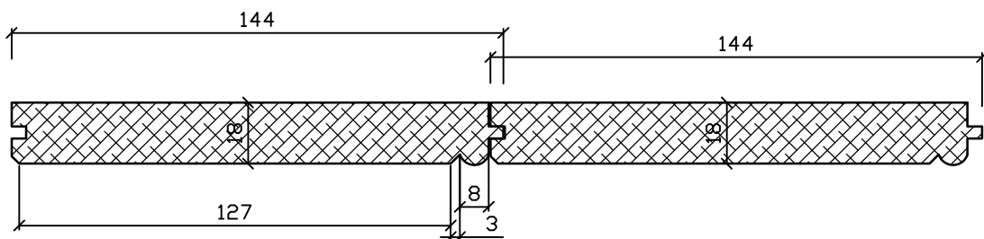
HORIZONTAL DETAIL through BEAD and BUTT WALL BOARDING - Scale 1:2 @ A1
