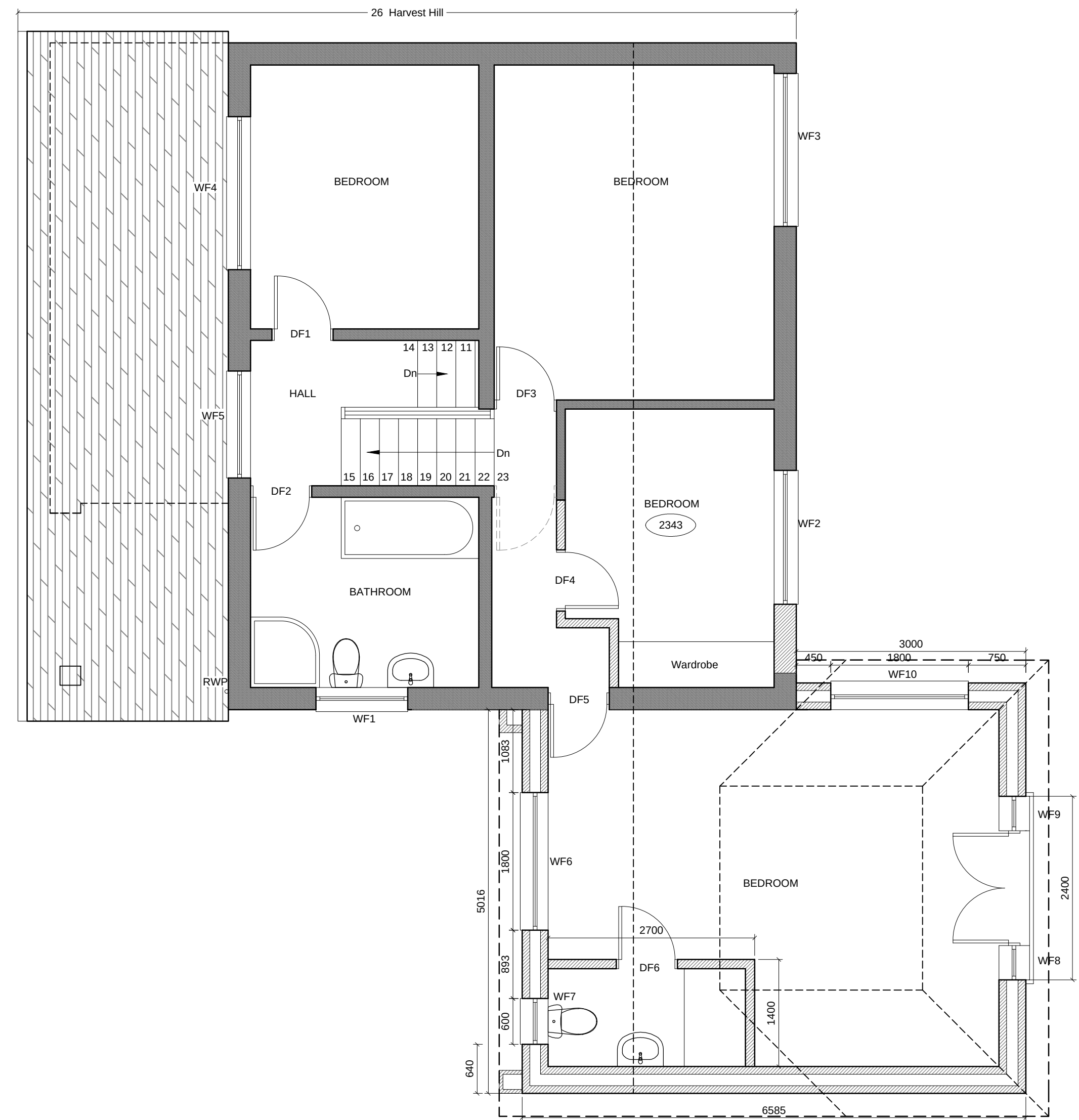
FIRST PLAN AS PROPOSED
