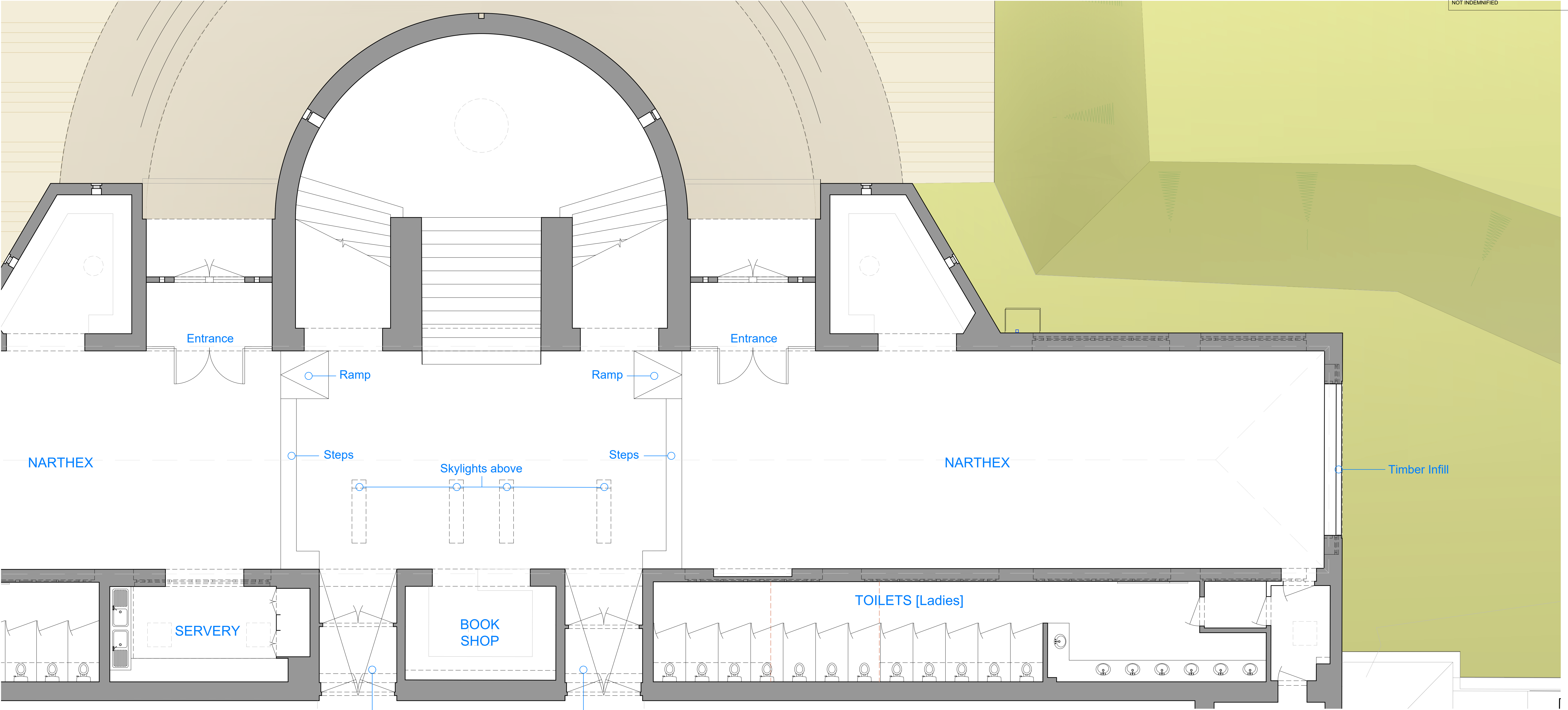
1. Existing Narthex 1:50 @ A1
