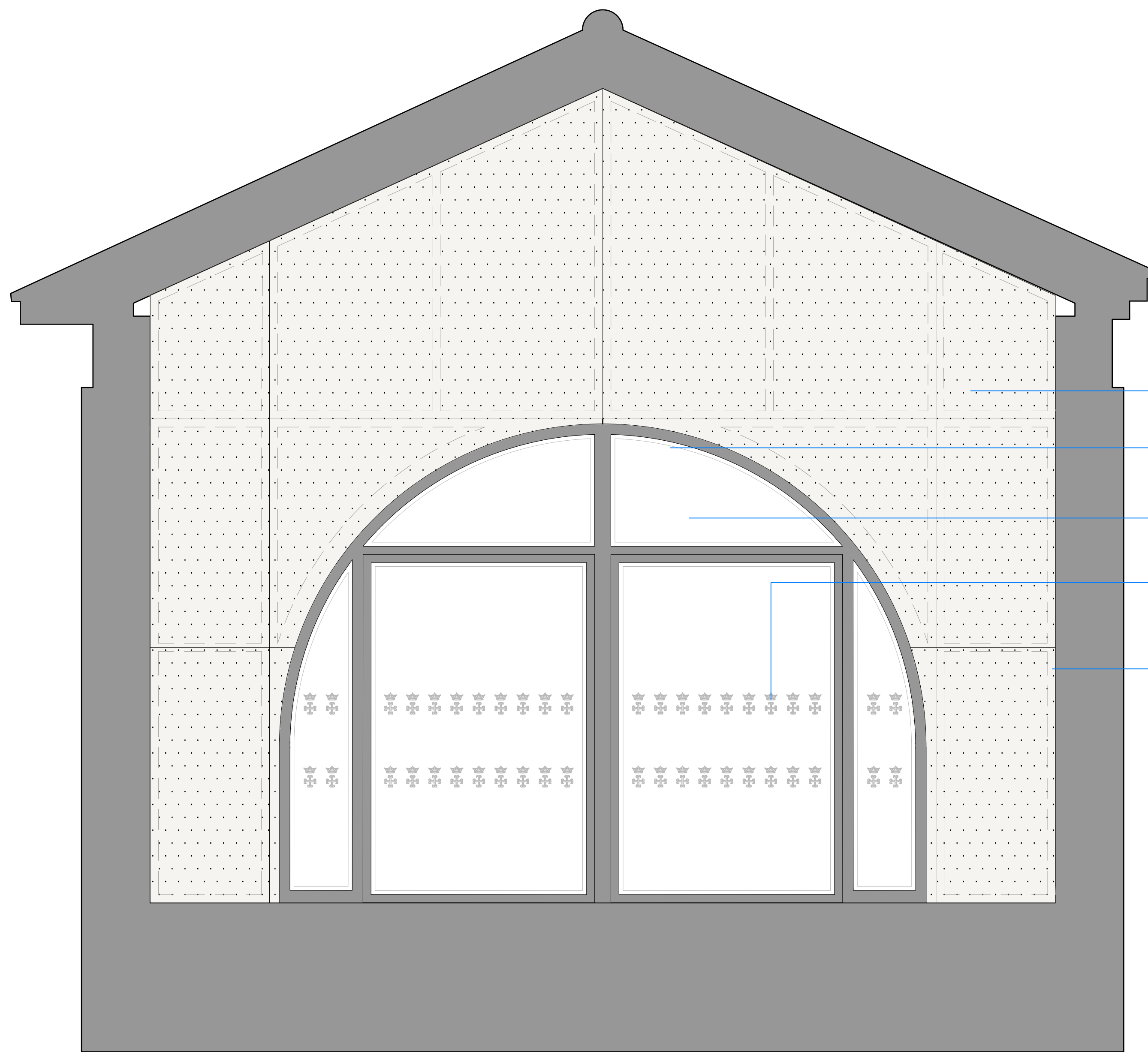
1. Proposed Narthex Section With Acoustic Screen
