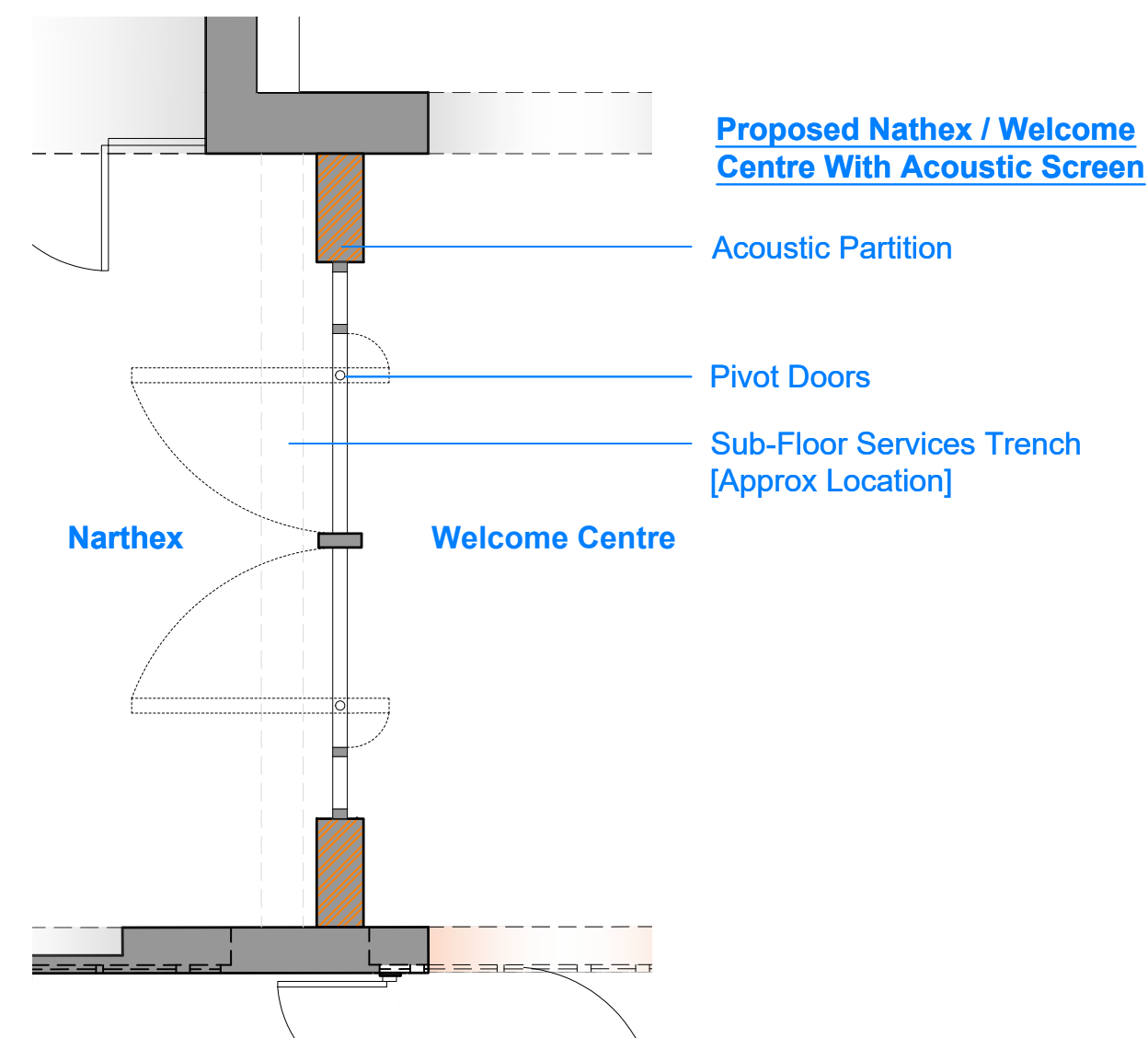
4. Proposed Acoustic Screen Plan
