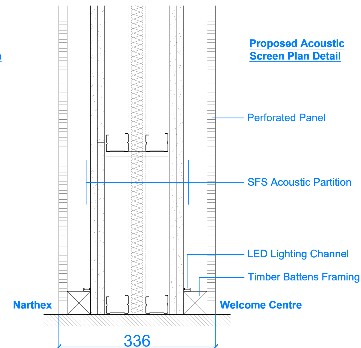
4. Proposed Acoustic Screen Plan
