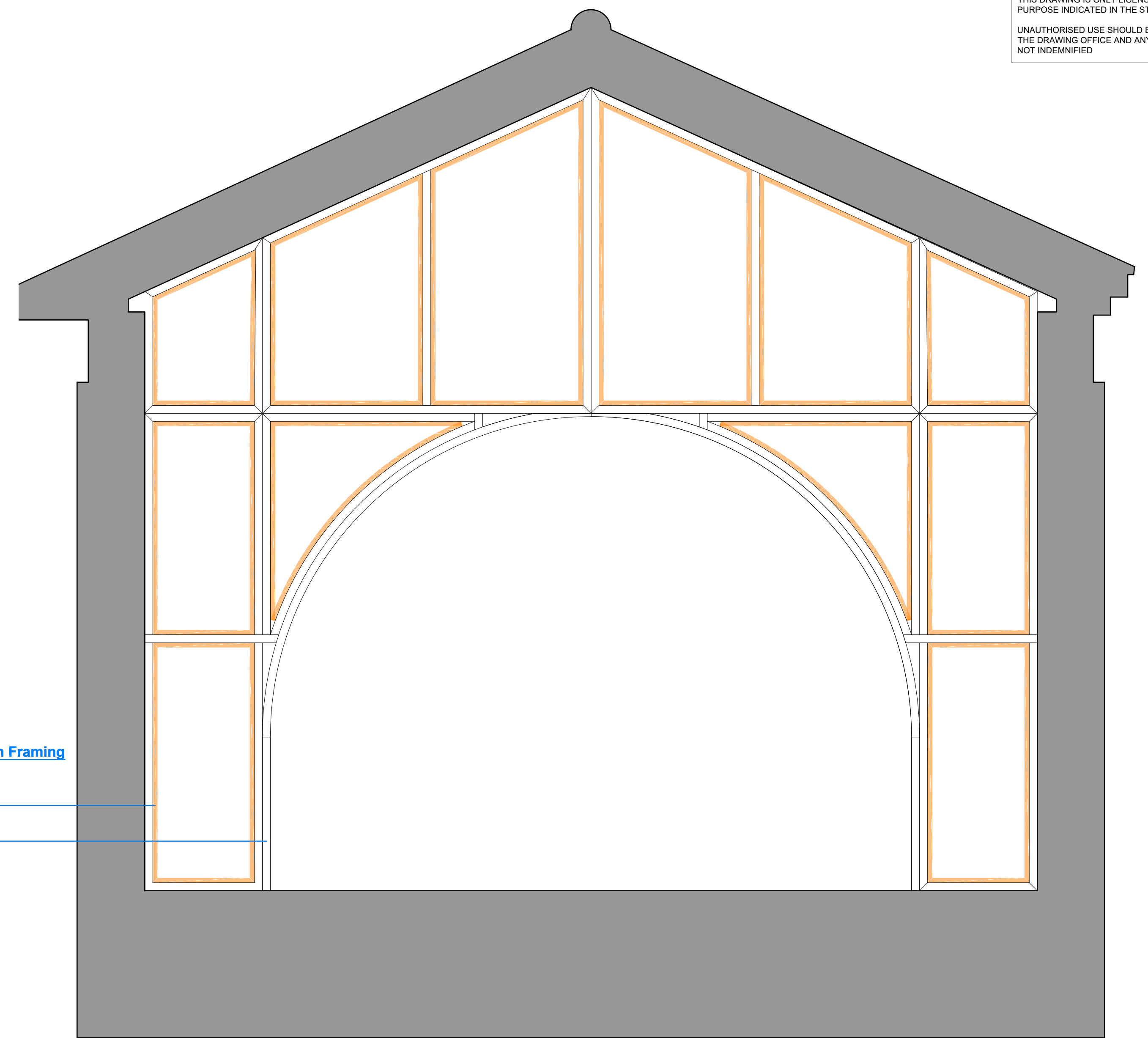
2. Proposed Narthex Section With Acoustic Screen Batten Layout
