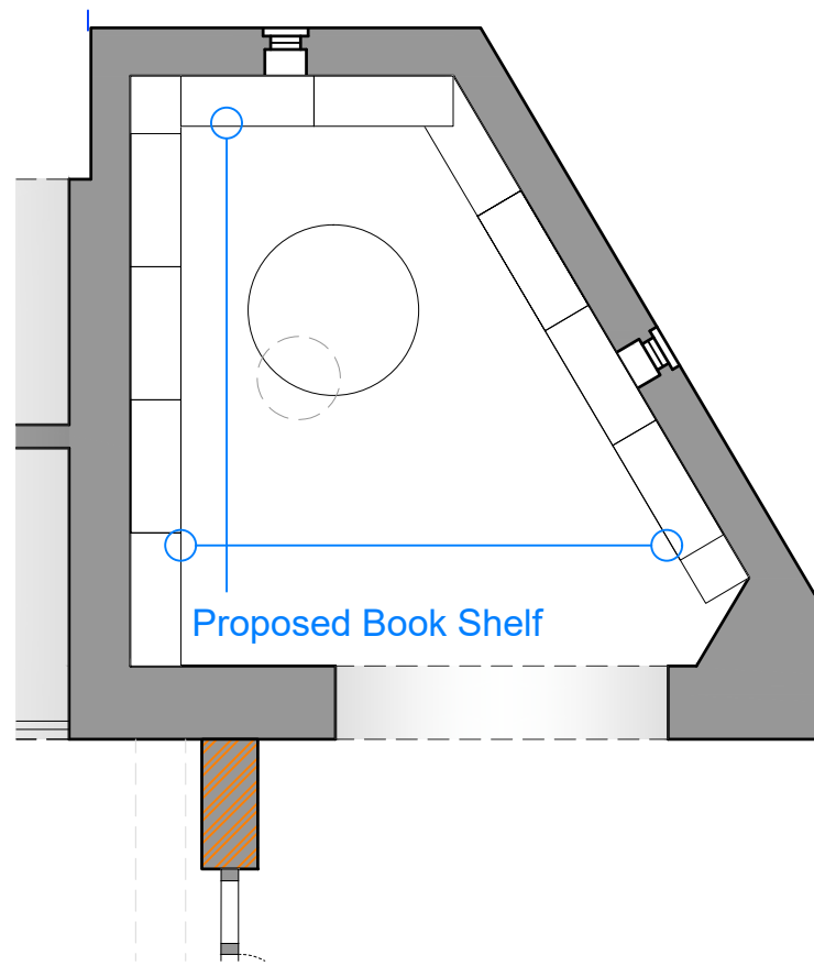
5. Proposed Study Plan 1:50 @ A1
