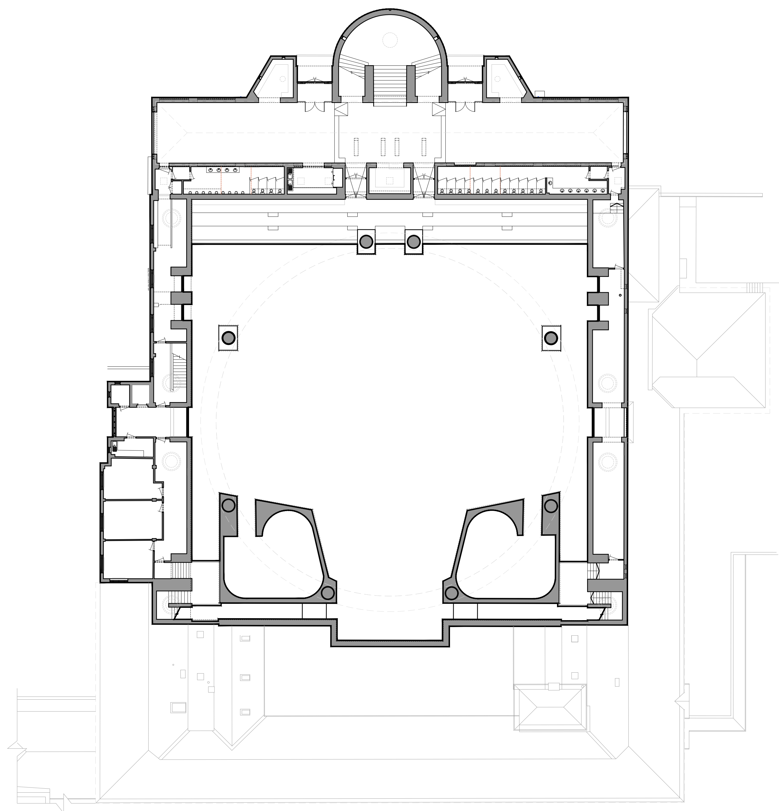
1. Existing Ground Floor GA Plan
