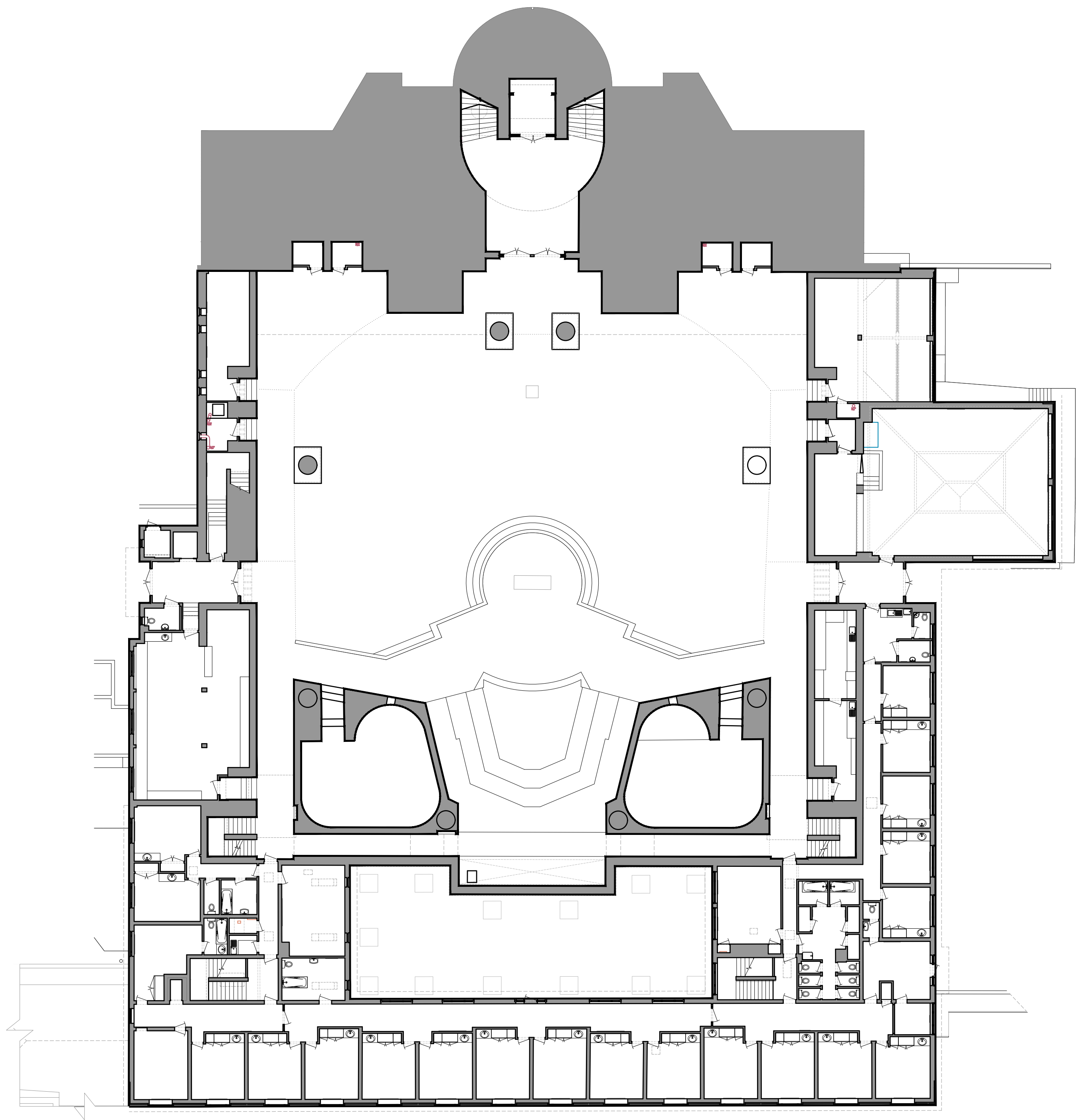
1. Existing Lower Ground Floor GA Plan 1:200 @ A1
