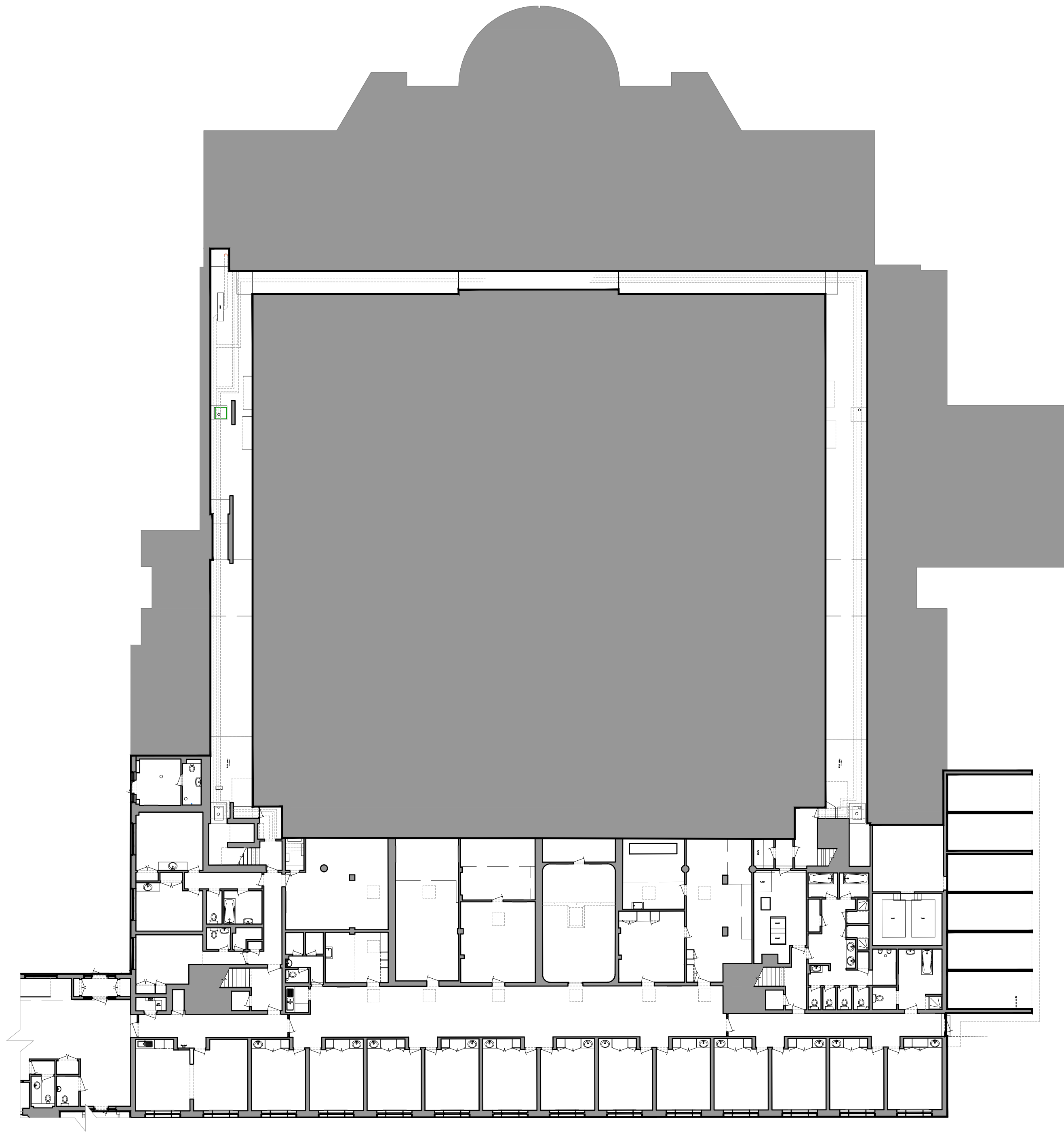
2. Existing Basement GA Plan 1:200 @ A1
