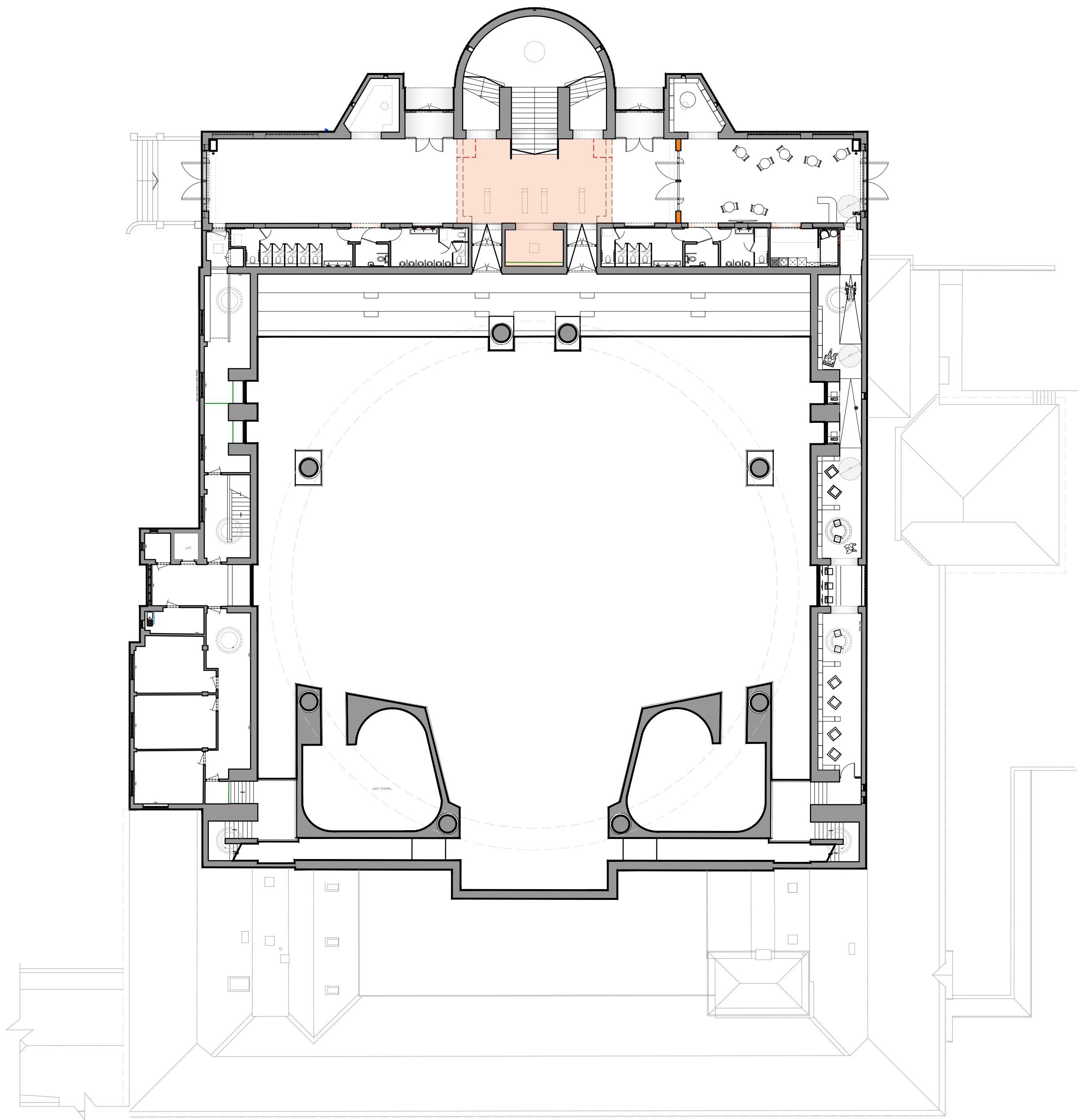
1. Existing Ground Floor GA Plan 1:200 @ A1
