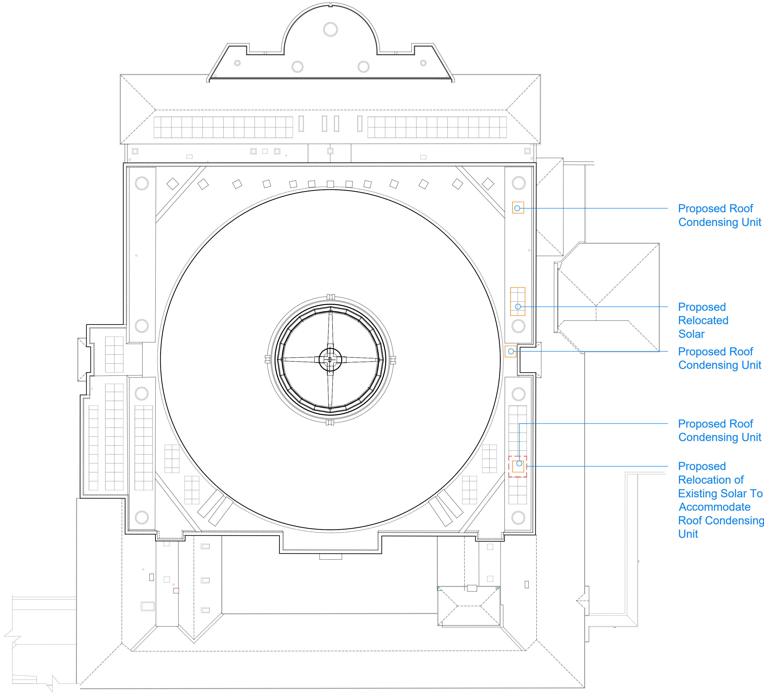
2. Existing Roof GA Plan 1:200 @ A1
