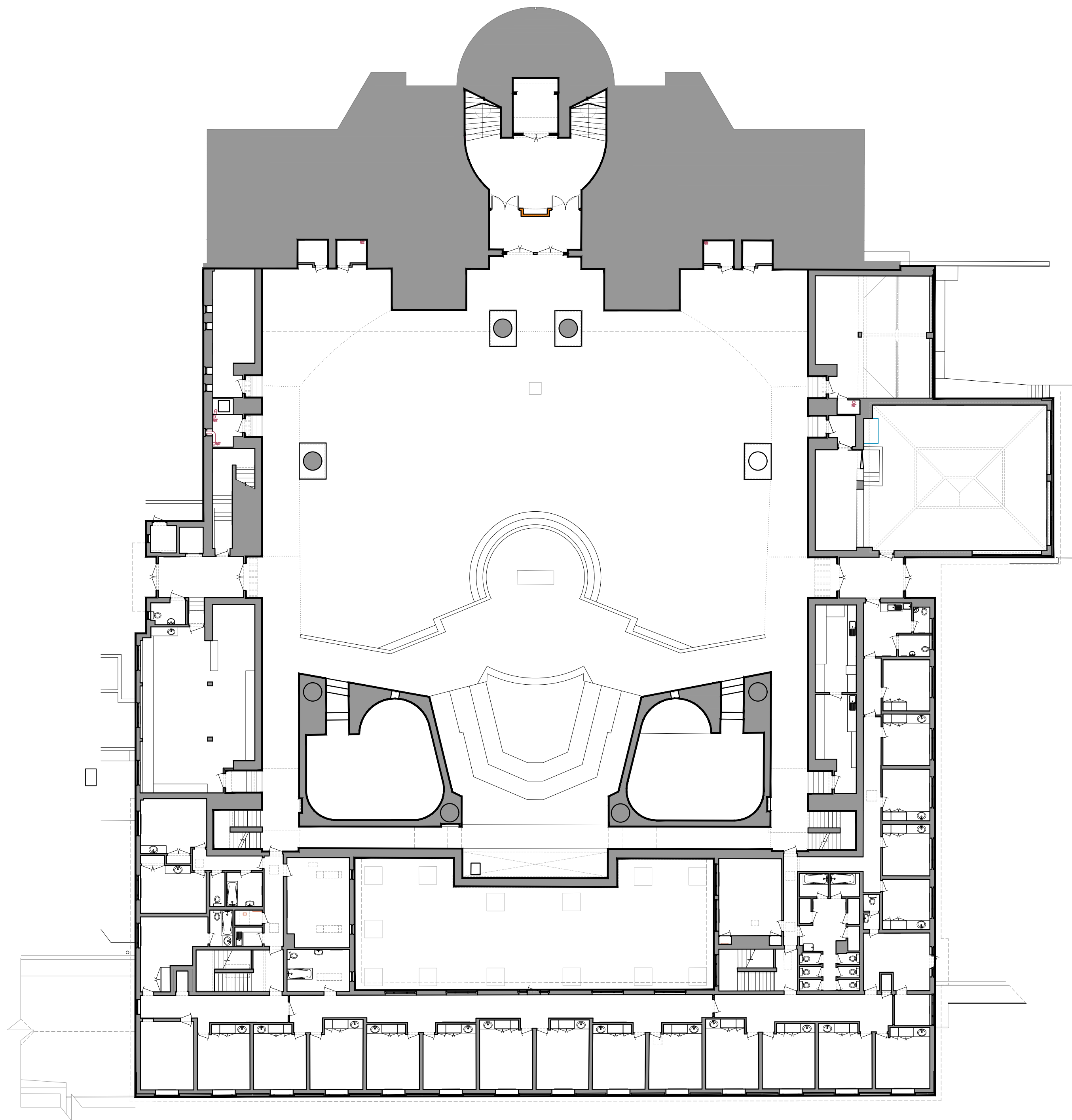
1. Proposed Lower Ground Floor GA Plan 1:200 @ A1
