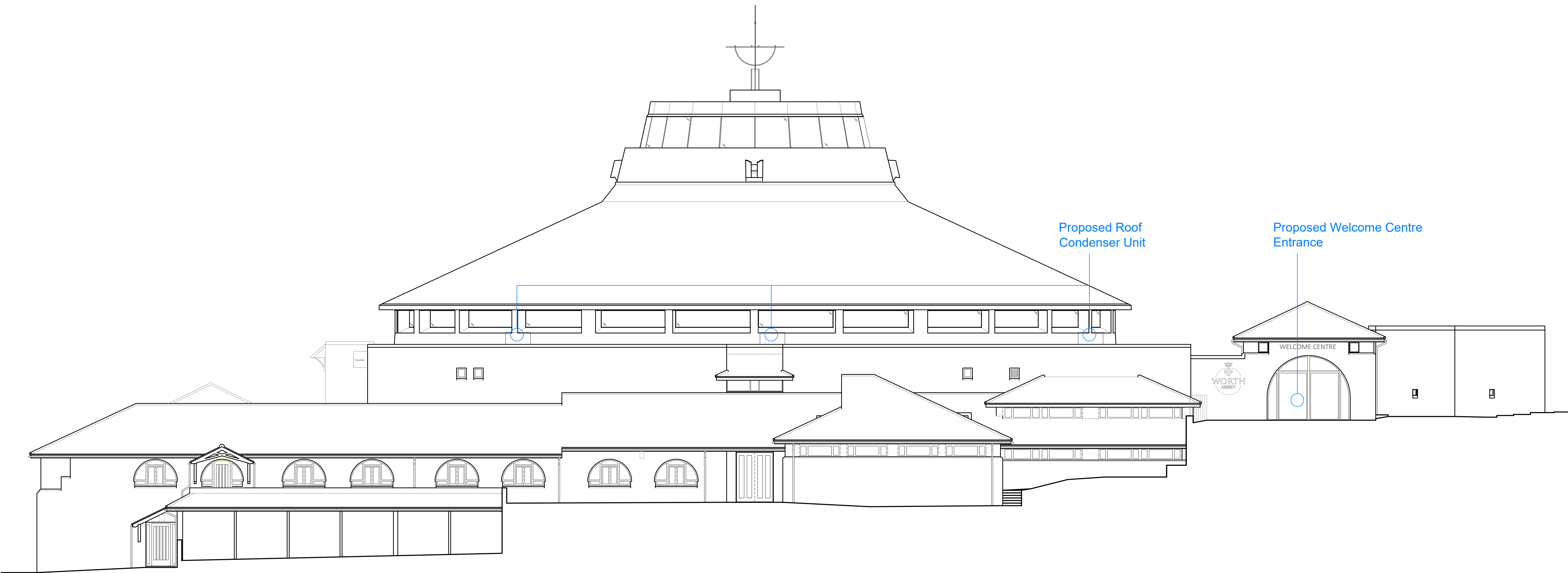
1. Proposed East Elevation 1:100 @ A1
