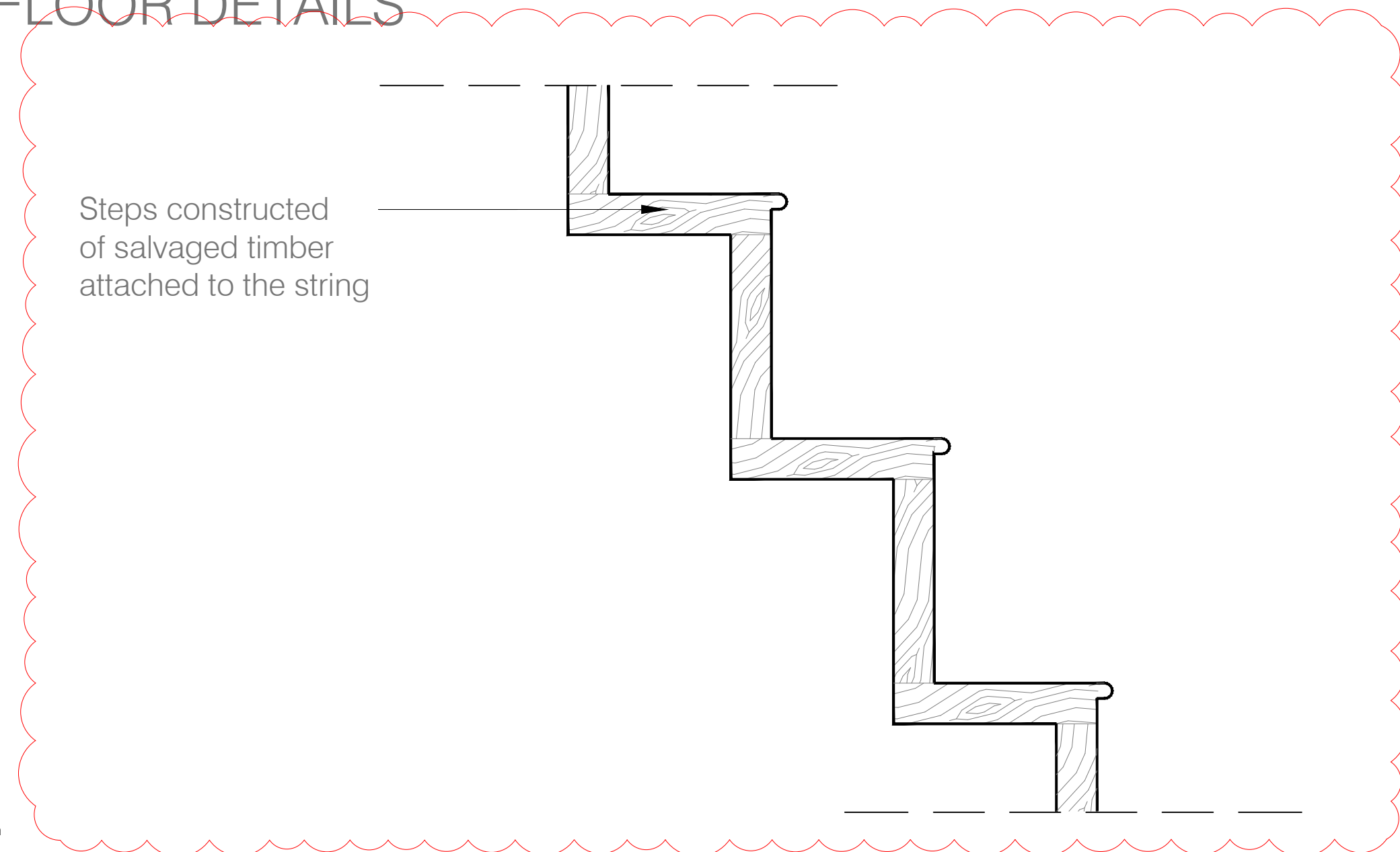
Detail 01 - Steps Section Scale 1:5@A1 1:10@A3
