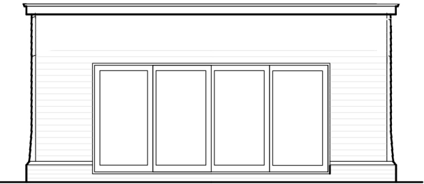
PROPOSED FRONT ELEVATION West facing
