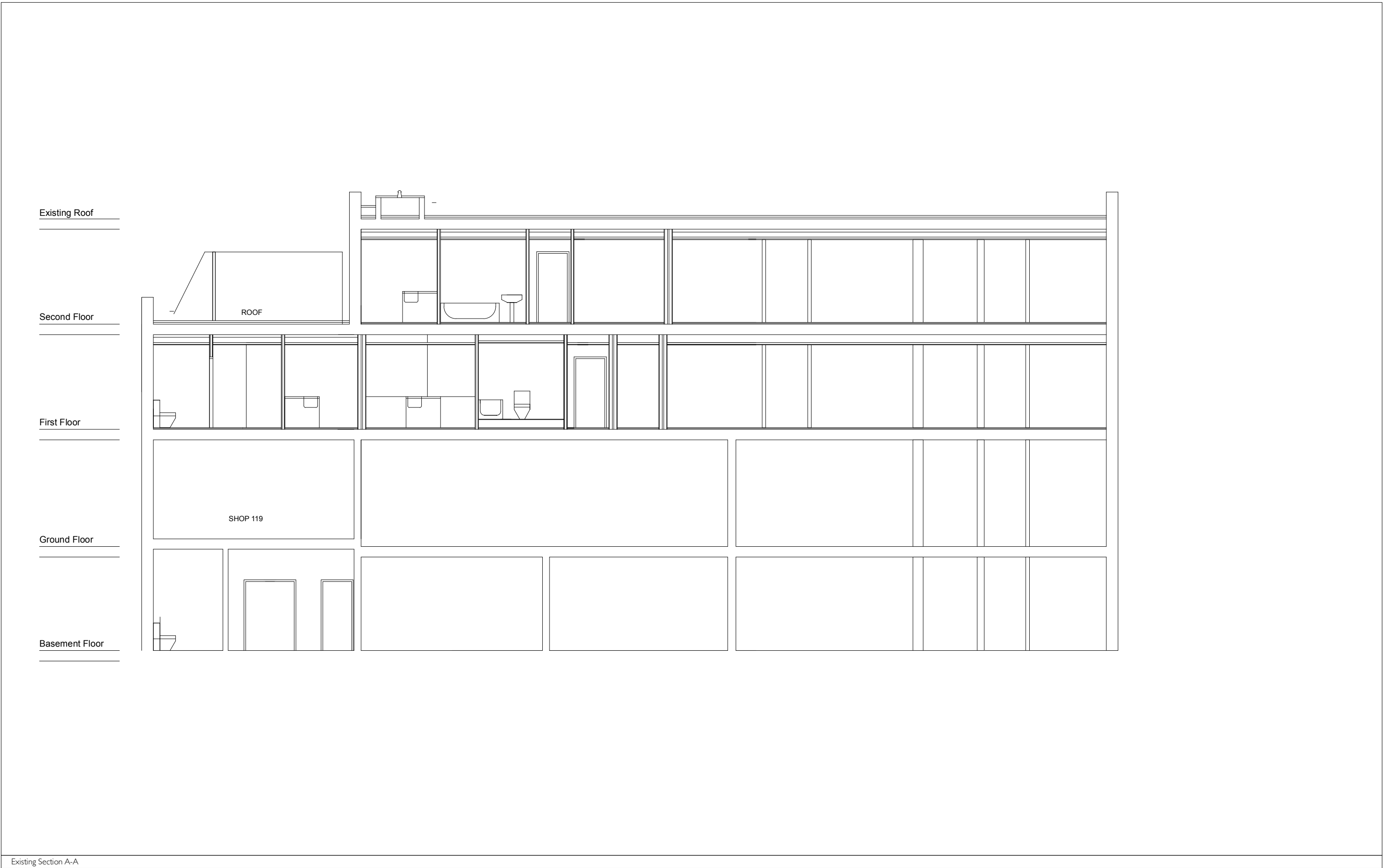
Existing Section A-A
