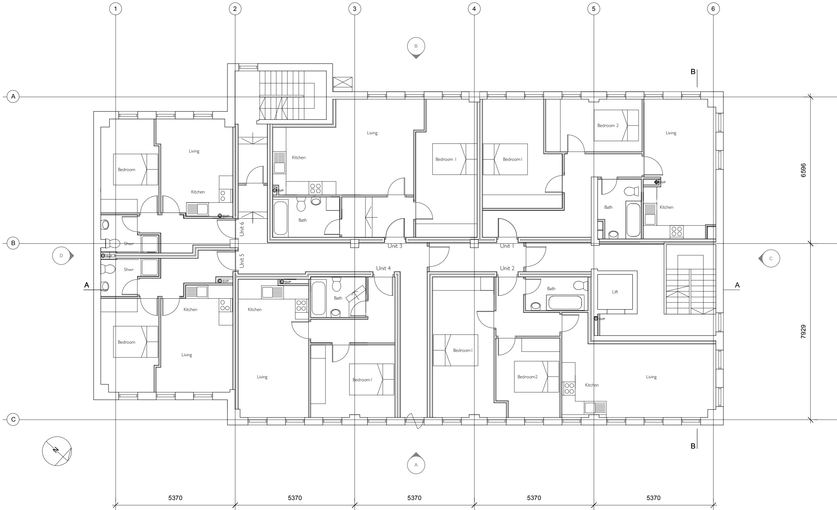
Proposed First Floor
