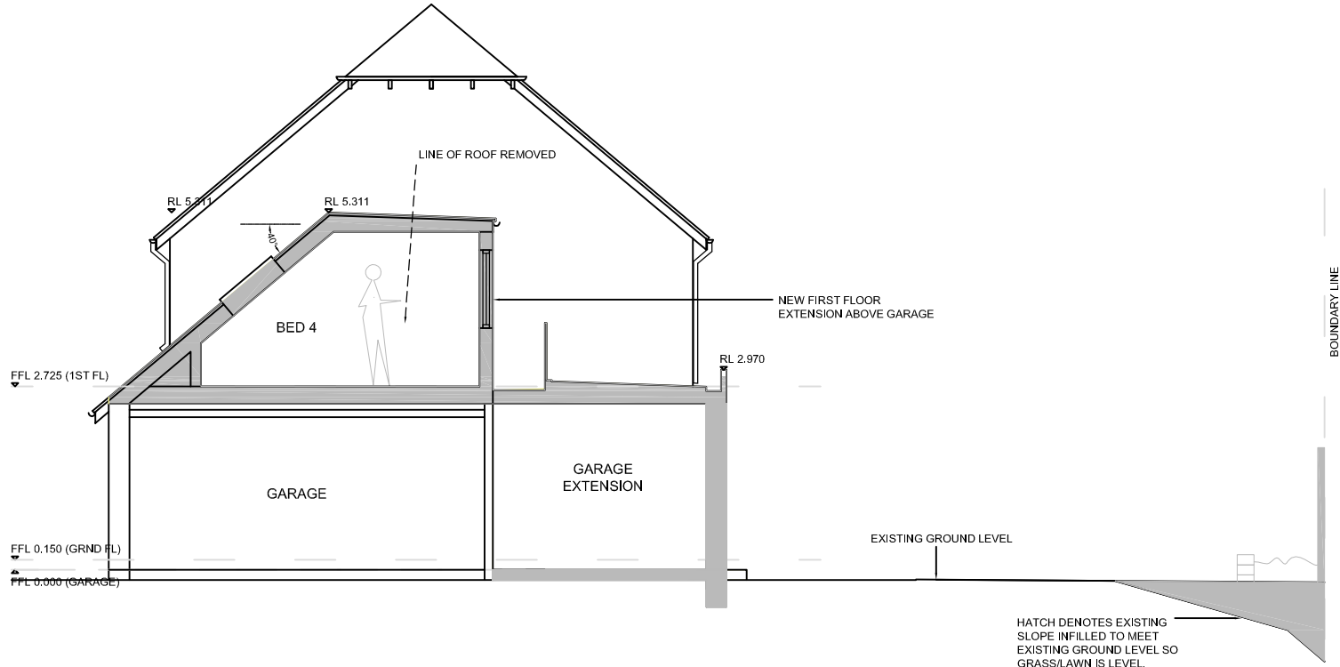
PROPOSED SECTION A
