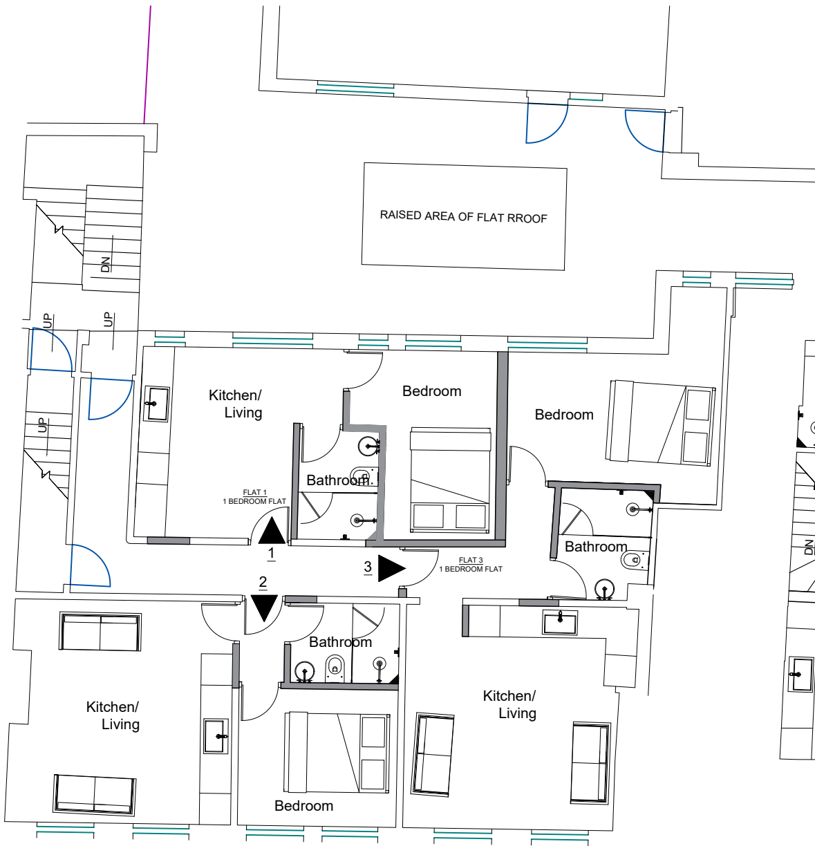
FIRST FLOOR
